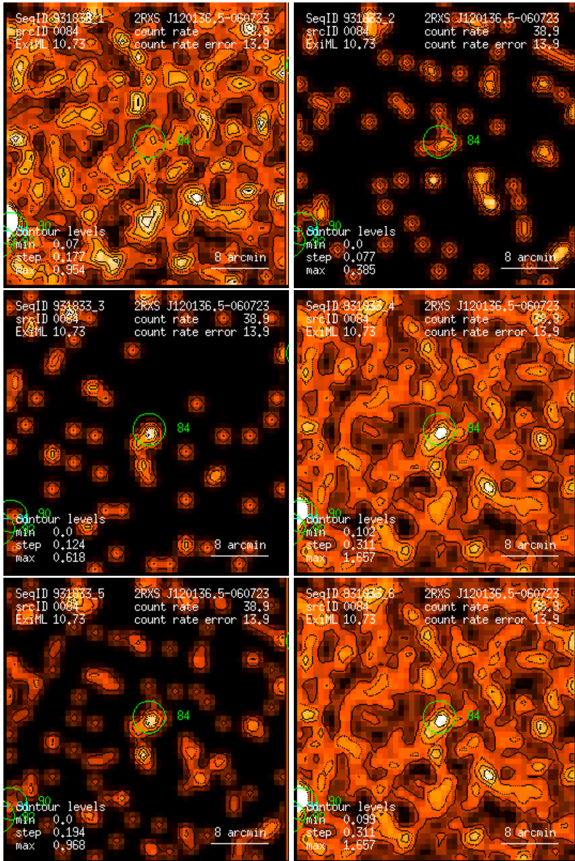
Figure 84: RASS 931833: detection 0084: band rate images, Gaussian filter: (1) PSPC channels 11 – 41, (2) 52 – 90, (3) 91 – 201, (4) 11 – 235, (5) 52 – 201, (6) 11 – 201. Broad band rates in counts/ks. Band rate contour levels in counts/ks/arcmin 2 .
