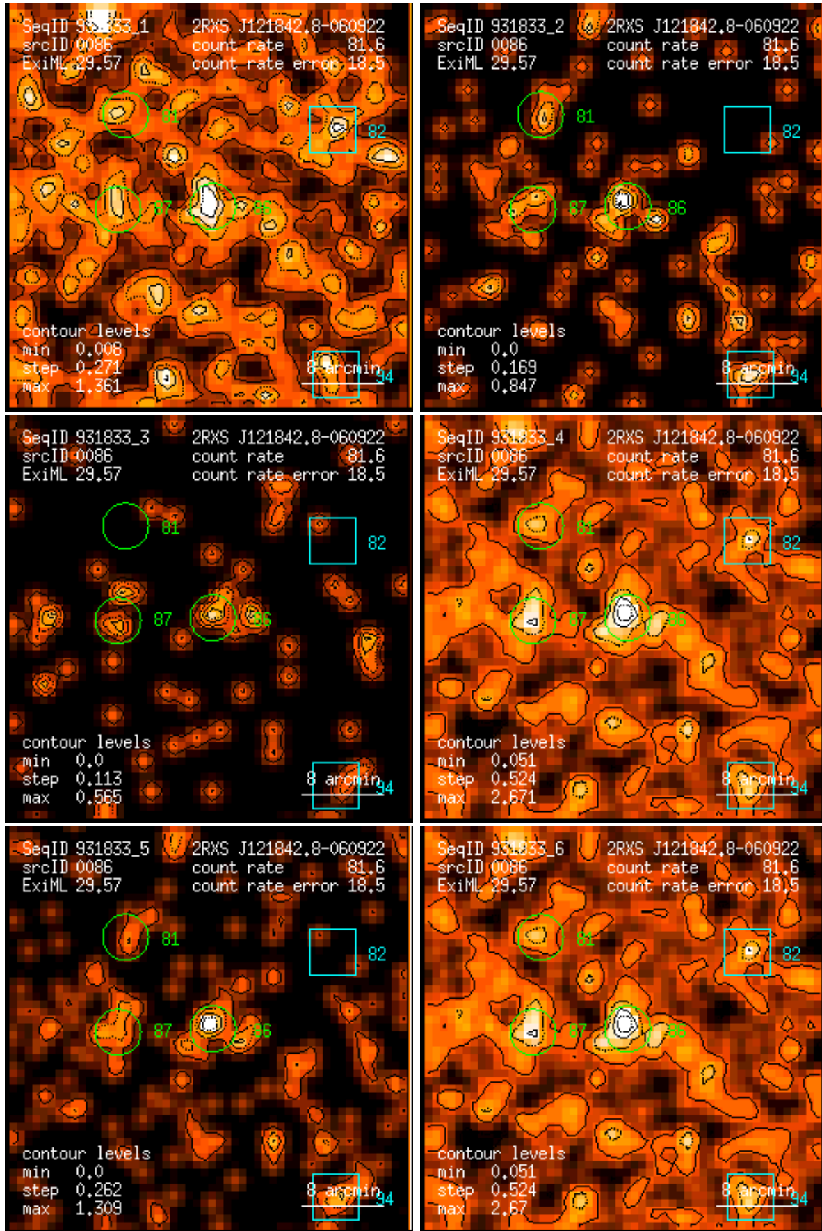
Figure 86: RASS 931833: detection 0086: band rate images, Gaussian filter: (1) PSPC channels 11 – 41, (2) 52 – 90, (3) 91 – 201, (4) 11 – 235, (5) 52 – 201, (6) 11 – 201. Broad band rates in counts/ks. Band rate contour levels in counts/ks/arcmin 2 .
