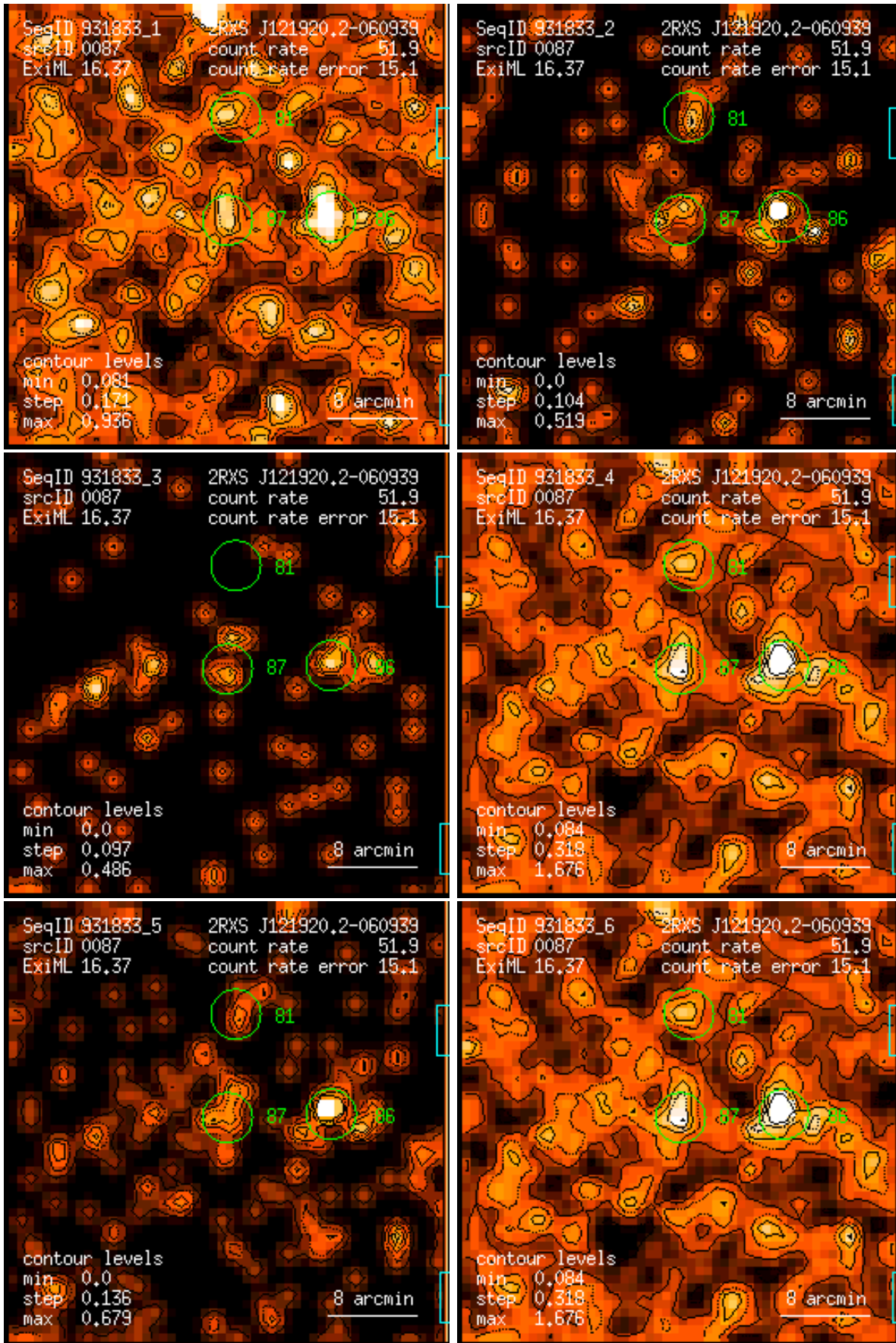
Figure 87: RASS 931833: detection 0087: band rate images, Gaussian filter: (1) PSPC channels 11 – 41, (2) 52 – 90, (3) 91 – 201, (4) 11 – 235, (5) 52 – 201, (6) 11 – 201. Broad band rates in counts/ks. Band rate contour levels in counts/ks/arcmin 2 .
