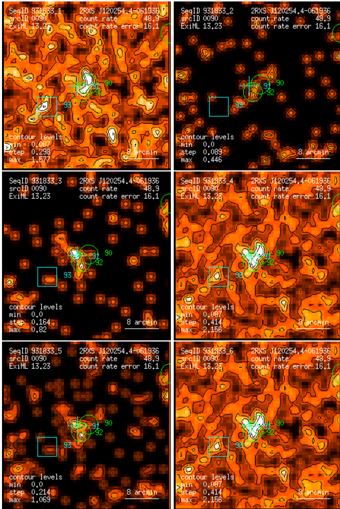
Figure 90: RASS 931833: detection 0090: band rate images, Gaussian filter: (1) PSPC channels 11 – 41, (2) 52 – 90, (3) 91 – 201, (4) 11 – 235, (5) 52 – 201, (6) 11 – 201. Broad band rates in counts/ks. Band rate contour levels in counts/ks/arcmin 2 .
