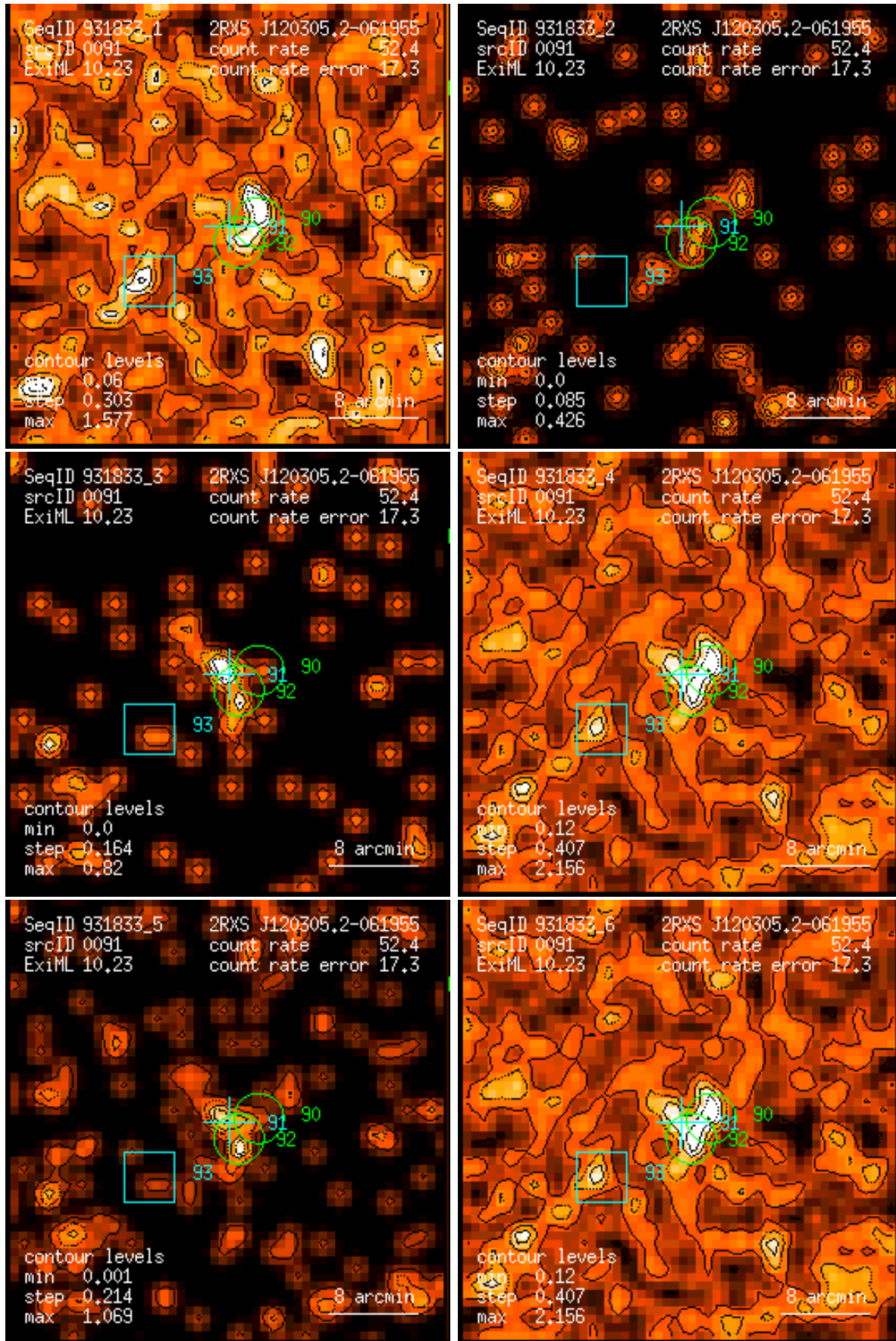
Figure 91: RASS 931833: detection 0091: band rate images, Gaussian filter: (1) PSPC channels 11 – 41, (2) 52 – 90, (3) 91 – 201, (4) 11 – 235, (5) 52 – 201, (6) 11 – 201. Broad band rates in counts/ks. Band rate contour levels in counts/ks/arcmin 2 .
