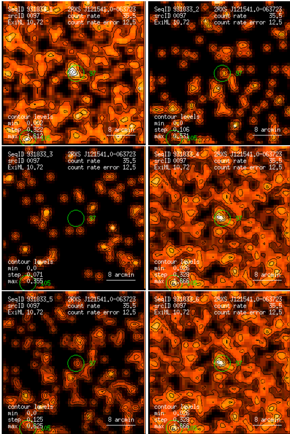
Figure 97: RASS 931833: detection 0097: band rate images, Gaussian filter: (1) PSPC channels 11 – 41, (2) 52 – 90, (3) 91 – 201, (4) 11 – 235, (5) 52 – 201, (6) 11 – 201. Broad band rates in counts/ks. Band rate contour levels in counts/ks/arcmin 2 .
