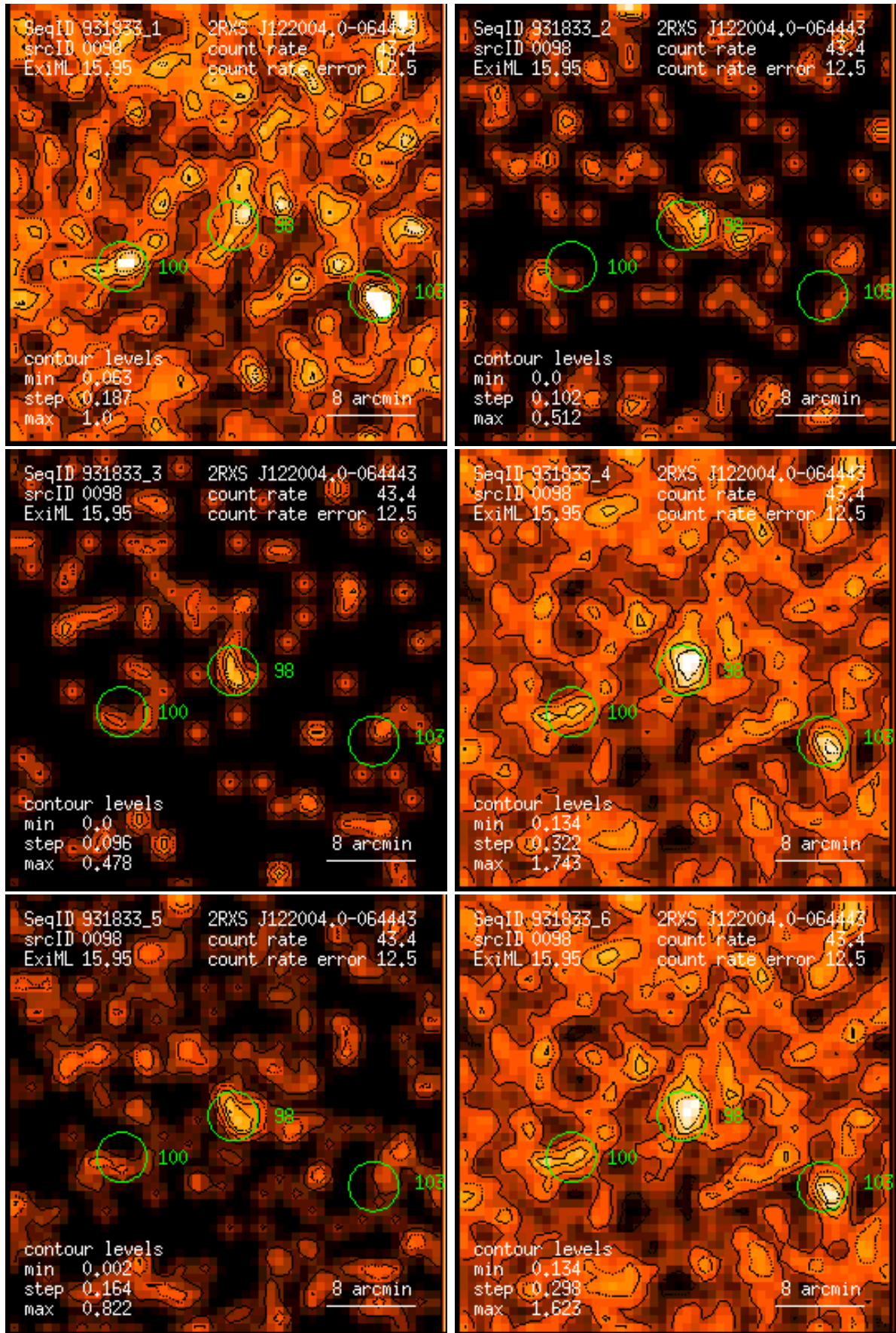
Figure 98: RASS 931833: detection 0098: band rate images, Gaussian filter: (1) PSPC channels 11 – 41, (2) 52 – 90, (3) 91 – 201, (4) 11 – 235, (5) 52 – 201, (6) 11 – 201. Broad band rates in counts/ks. Band rate contour levels in counts/ks/arcmin 2 .
