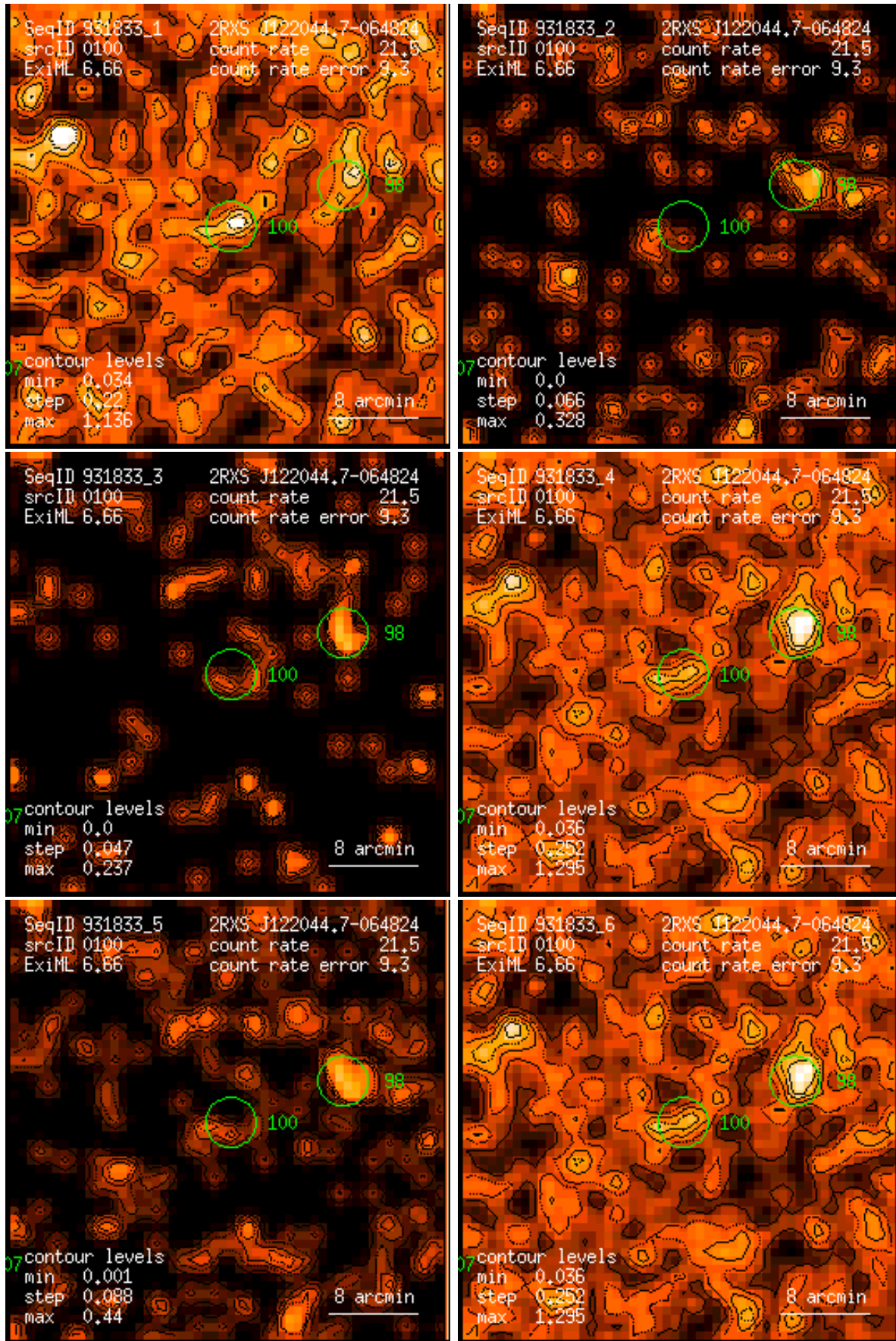
Figure 100: RASS 931833: detection 0100: band rate images, Gaussian filter: (1) PSPC channels 11 – 41, (2) 52 – 90, (3) 91 – 201, (4) 11 – 235, (5) 52 – 201, (6) 11 – 201. Broad band rates in counts/ks. Band rate contour levels in counts/ks/arcmin 2 .
