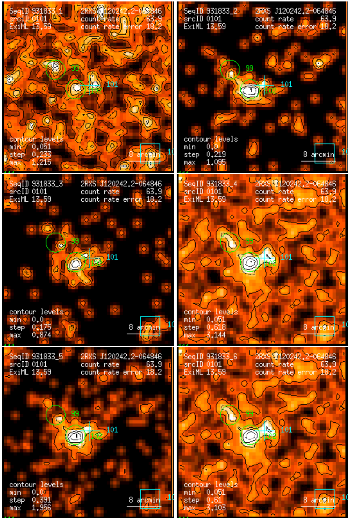
Figure 101: RASS 931833: detection 0101: band rate images, Gaussian filter: (1) PSPC channels 11 – 41, (2) 52 – 90, (3) 91 – 201, (4) 11 – 235, (5) 52 – 201, (6) 11 – 201. Broad band rates in counts/ks. Band rate contour levels in counts/ks/arcmin 2 .
