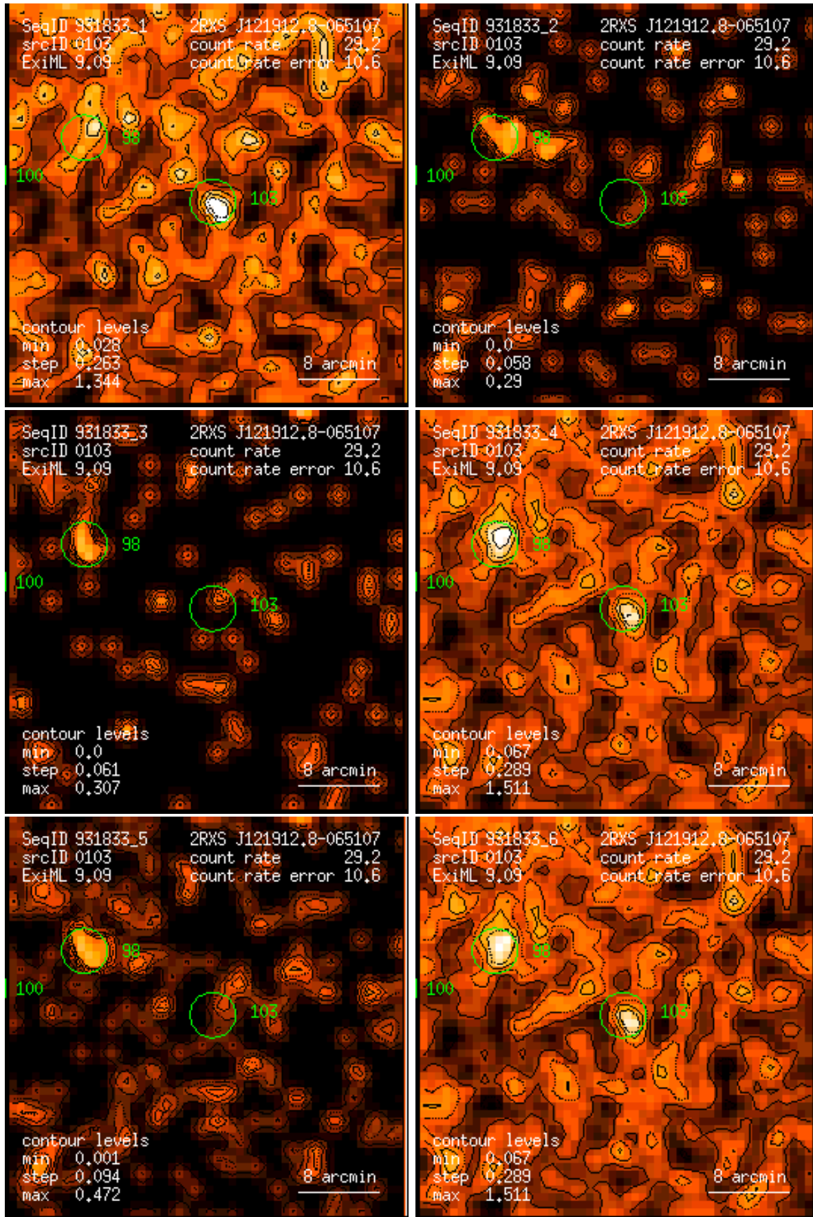
Figure 103: RASS 931833: detection 0103: band rate images, Gaussian filter: (1) PSPC channels 11 – 41, (2) 52 – 90, (3) 91 – 201, (4) 11 – 235, (5) 52 – 201, (6) 11 – 201. Broad band rates in counts/ks. Band rate contour levels in counts/ks/arcmin 2 .
