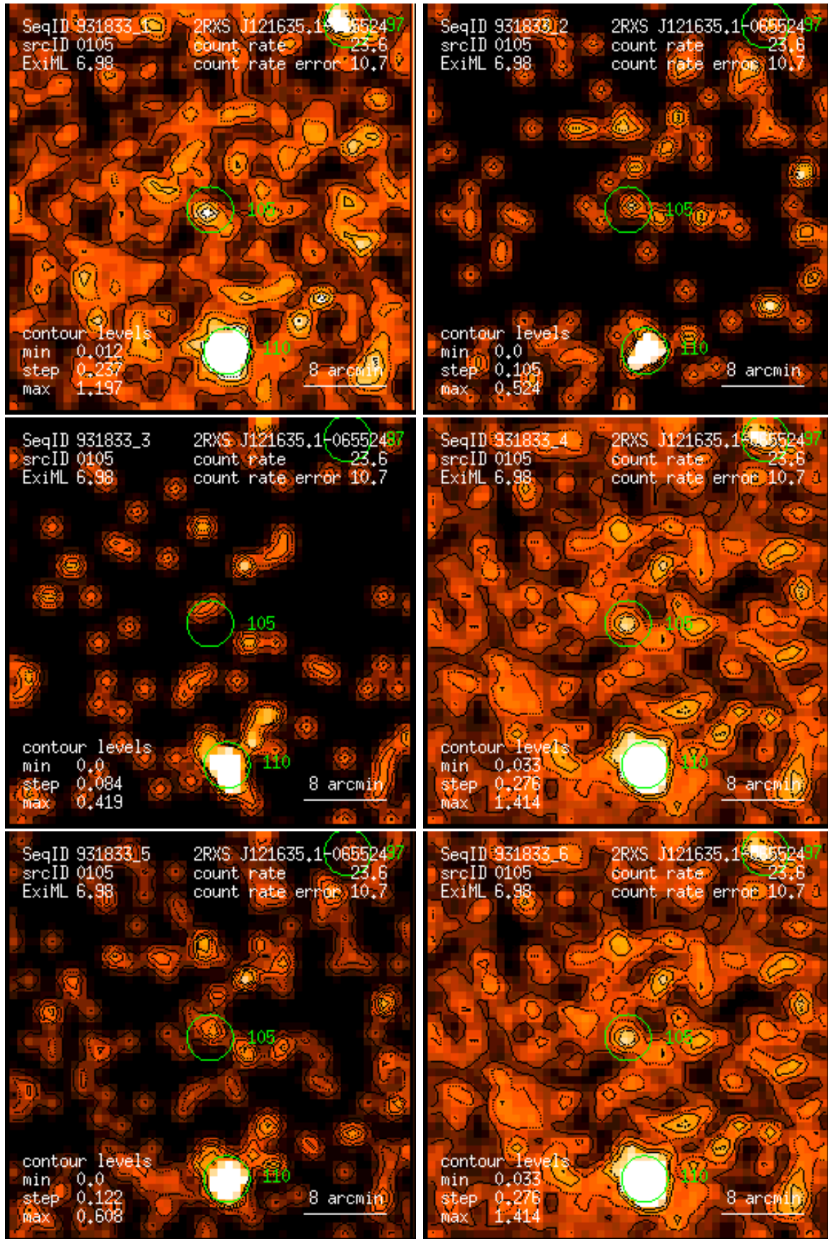
Figure 105: RASS 931833: detection 0105: band rate images, Gaussian filter: (1) PSPC channels 11 – 41, (2) 52 – 90, (3) 91 – 201, (4) 11 – 235, (5) 52 – 201, (6) 11 – 201. Broad band rates in counts/ks. Band rate contour levels in counts/ks/arcmin 2 .
