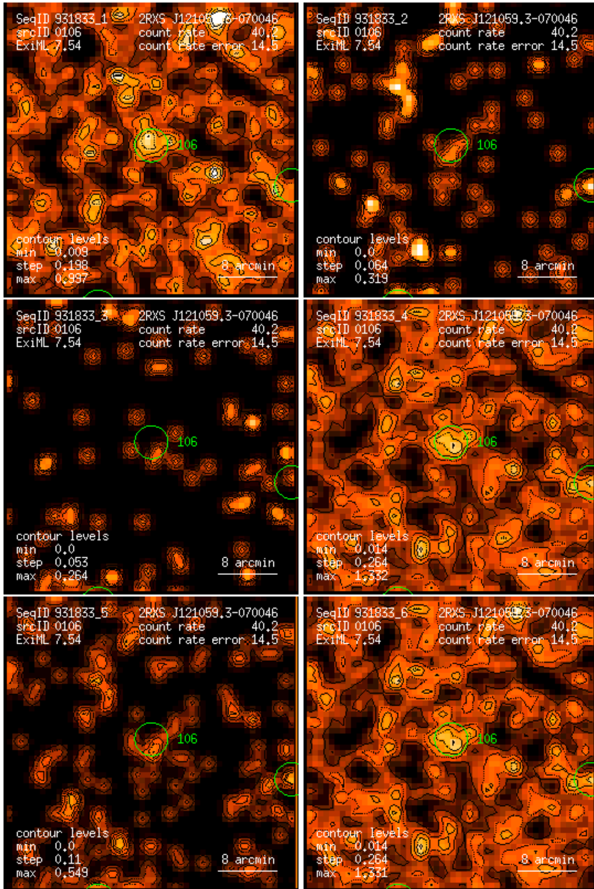
Figure 106: RASS 931833: detection 0106: band rate images, Gaussian filter: (1) PSPC channels 11 – 41, (2) 52 – 90, (3) 91 – 201, (4) 11 – 235, (5) 52 – 201, (6) 11 – 201. Broad band rates in counts/ks. Band rate contour levels in counts/ks/arcmin 2 .
