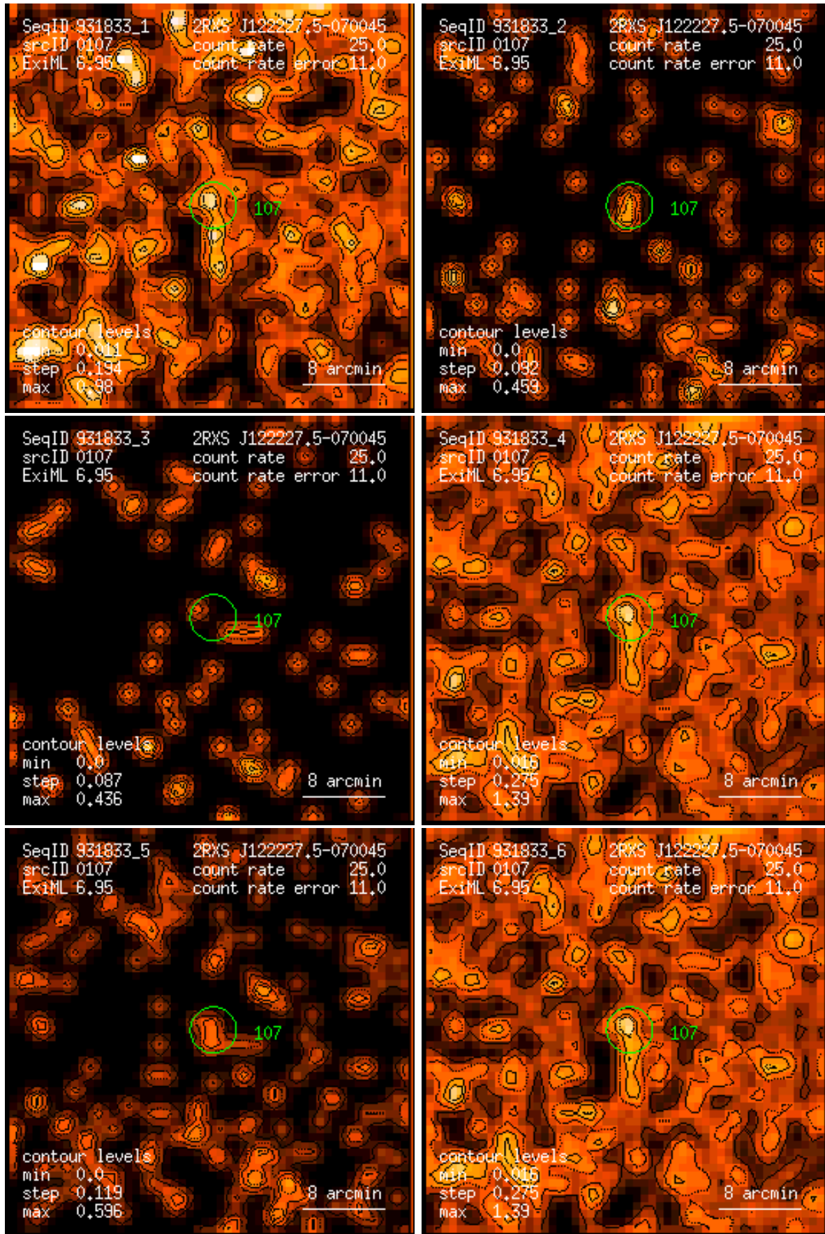
Figure 107: RASS 931833: detection 0107: band rate images, Gaussian filter: (1) PSPC channels 11 – 41, (2) 52 – 90, (3) 91 – 201, (4) 11 – 235, (5) 52 – 201, (6) 11 – 201. Broad band rates in counts/ks. Band rate contour levels in counts/ks/arcmin 2 .
