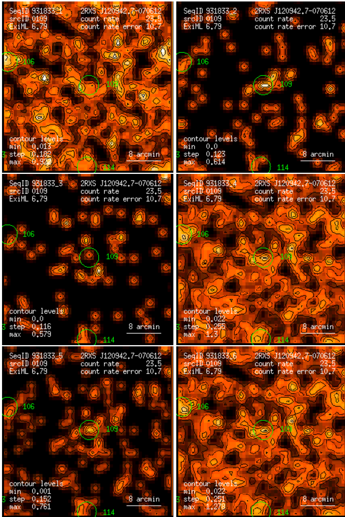
Figure 109: RASS 931833: detection 0109: band rate images, Gaussian filter: (1) PSPC channels 11 – 41, (2) 52 – 90, (3) 91 – 201, (4) 11 – 235, (5) 52 – 201, (6) 11 – 201. Broad band rates in counts/ks. Band rate contour levels in counts/ks/arcmin 2 .
