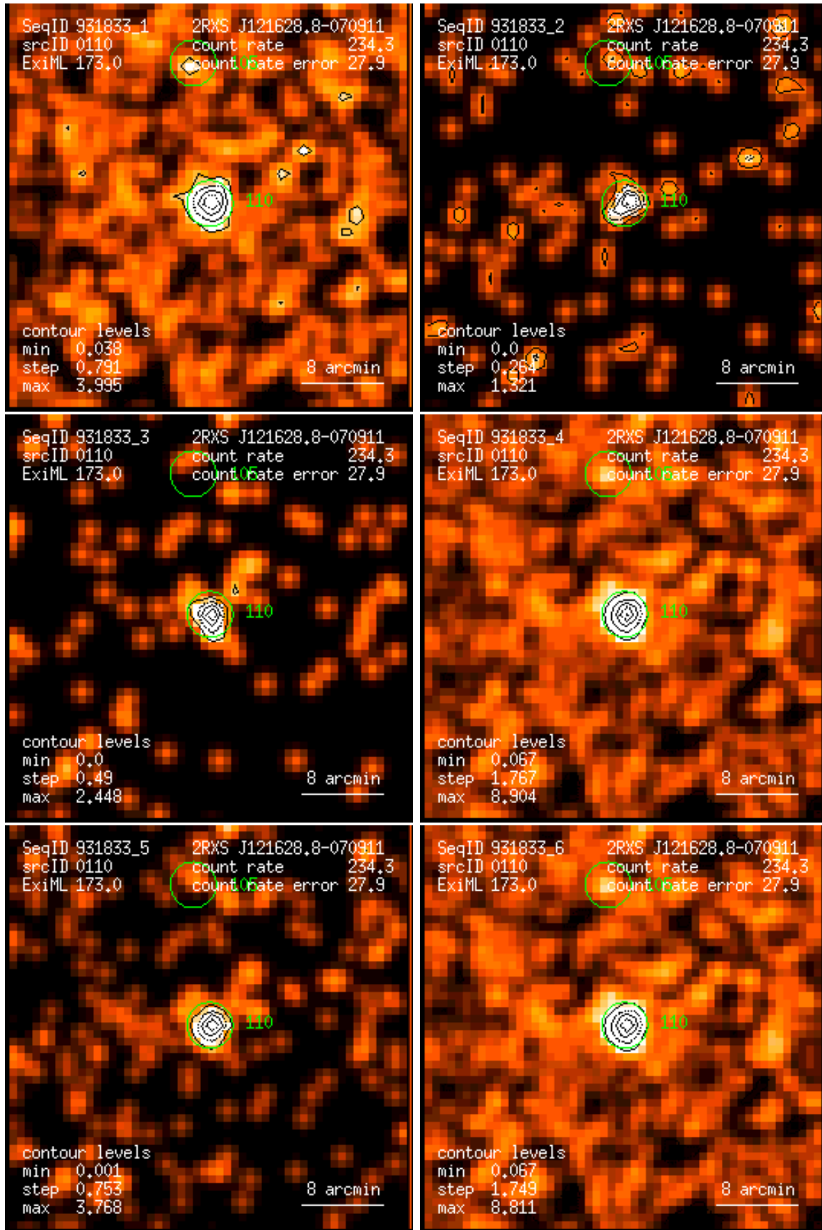
Figure 110: RASS 931833: detection 0110: band rate images, Gaussian filter: (1) PSPC channels 11 – 41, (2) 52 – 90, (3) 91 – 201, (4) 11 – 235, (5) 52 – 201, (6) 11 – 201. Broad band rates in counts/ks. Band rate contour levels in counts/ks/arcmin 2 .
