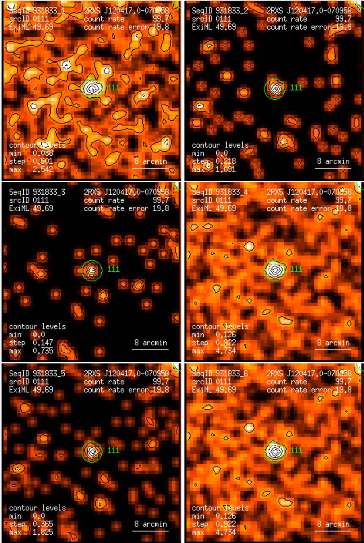
Figure 111: RASS 931833: detection 0111: band rate images, Gaussian filter: (1) PSPC channels 11 – 41, (2) 52 – 90, (3) 91 – 201, (4) 11 – 235, (5) 52 – 201, (6) 11 – 201. Broad band rates in counts/ks. Band rate contour levels in counts/ks/arcmin 2 .
