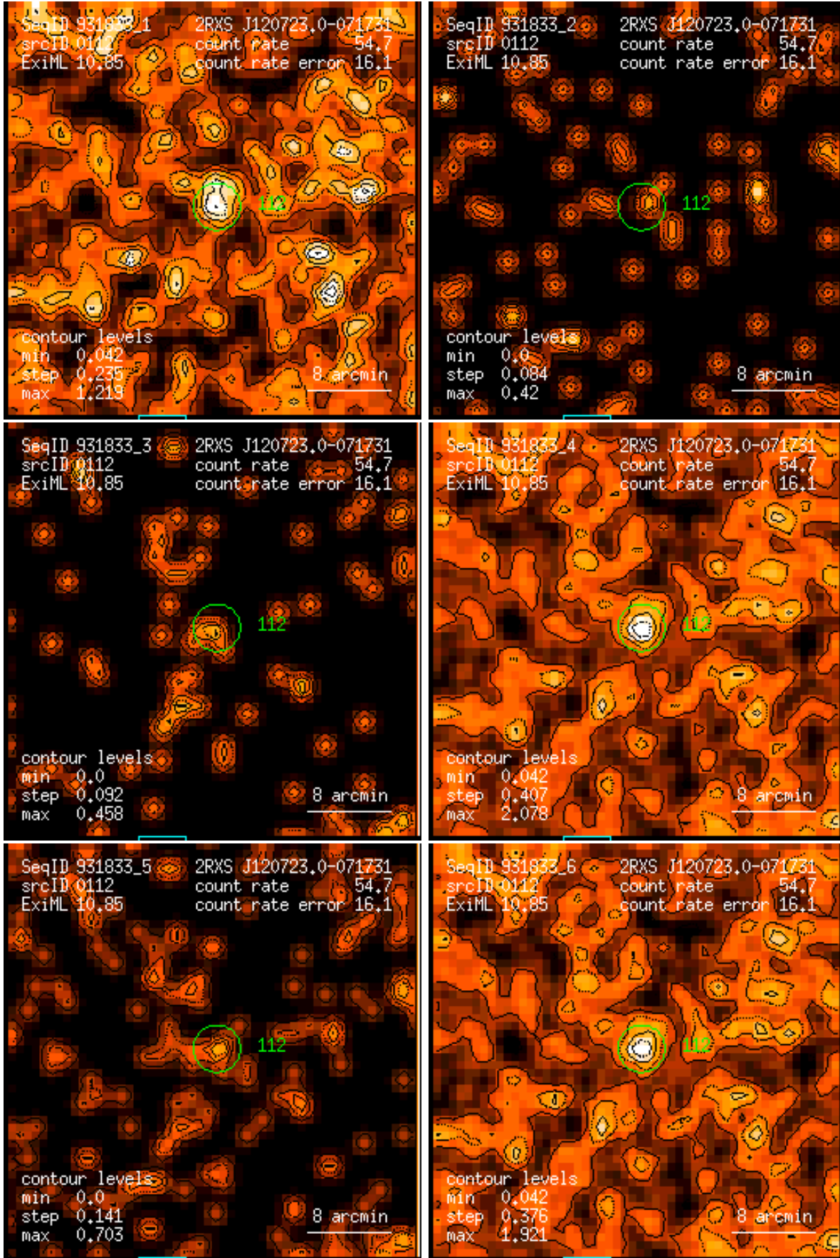
Figure 112: RASS 931833: detection 0112: band rate images, Gaussian filter: (1) PSPC channels 11 – 41, (2) 52 – 90, (3) 91 – 201, (4) 11 – 235, (5) 52 – 201, (6) 11 – 201. Broad band rates in counts/ks. Band rate contour levels in counts/ks/arcmin 2 .
