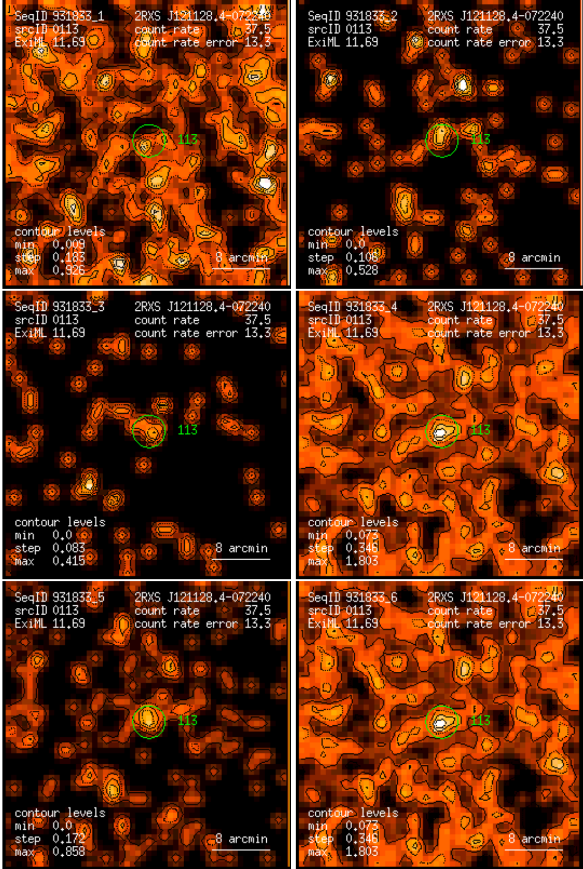
Figure 113: RASS 931833: detection 0113: band rate images, Gaussian filter: (1) PSPC channels 11 – 41, (2) 52 – 90, (3) 91 – 201, (4) 11 – 235, (5) 52 – 201, (6) 11 – 201. Broad band rates in counts/ks. Band rate contour levels in counts/ks/arcmin 2 .
