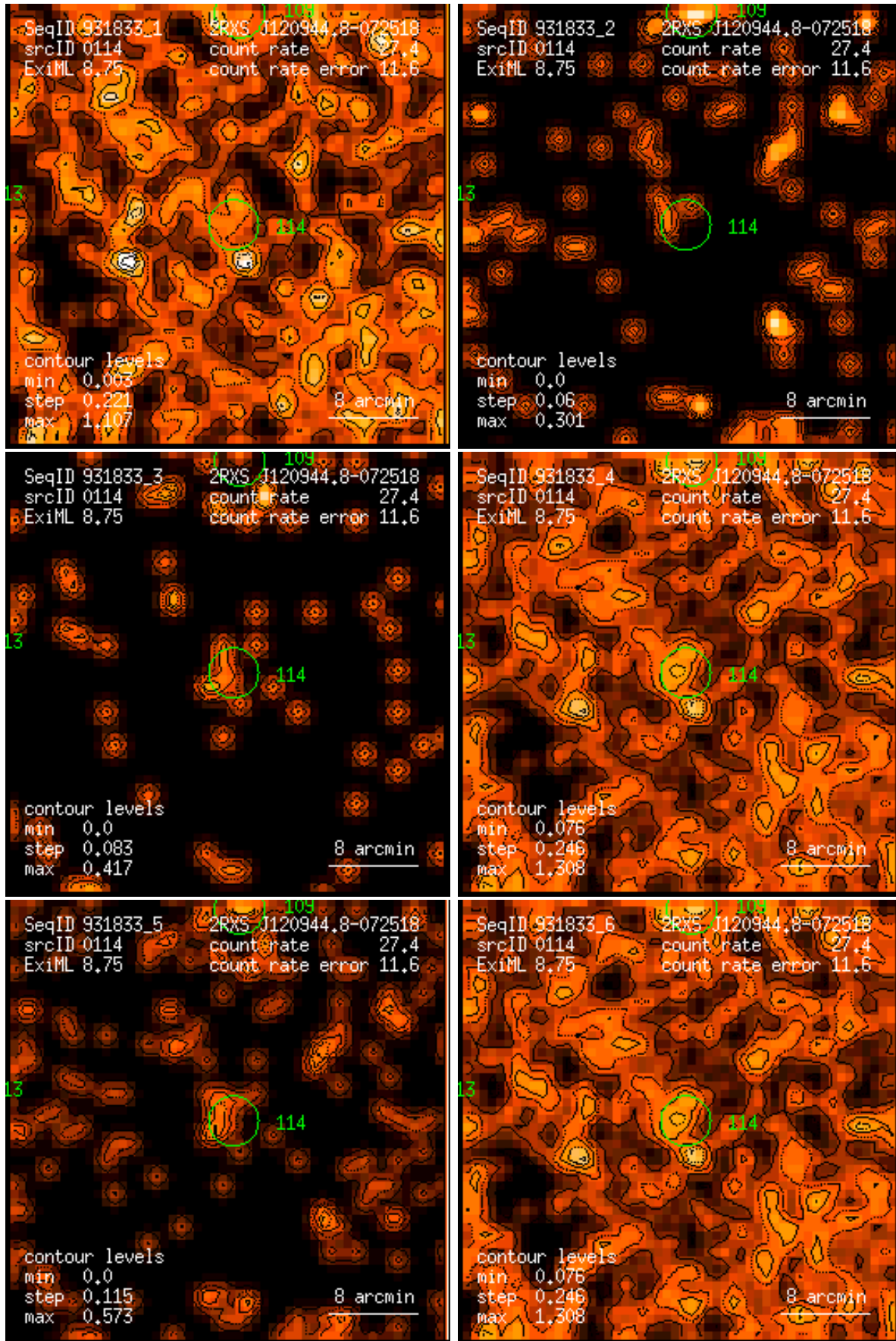
Figure 114: RASS 931833: detection 0114: band rate images, Gaussian filter: (1) PSPC channels 11 – 41, (2) 52 – 90, (3) 91 – 201, (4) 11 – 235, (5) 52 – 201, (6) 11 – 201. Broad band rates in counts/ks. Band rate contour levels in counts/ks/arcmin 2 .
