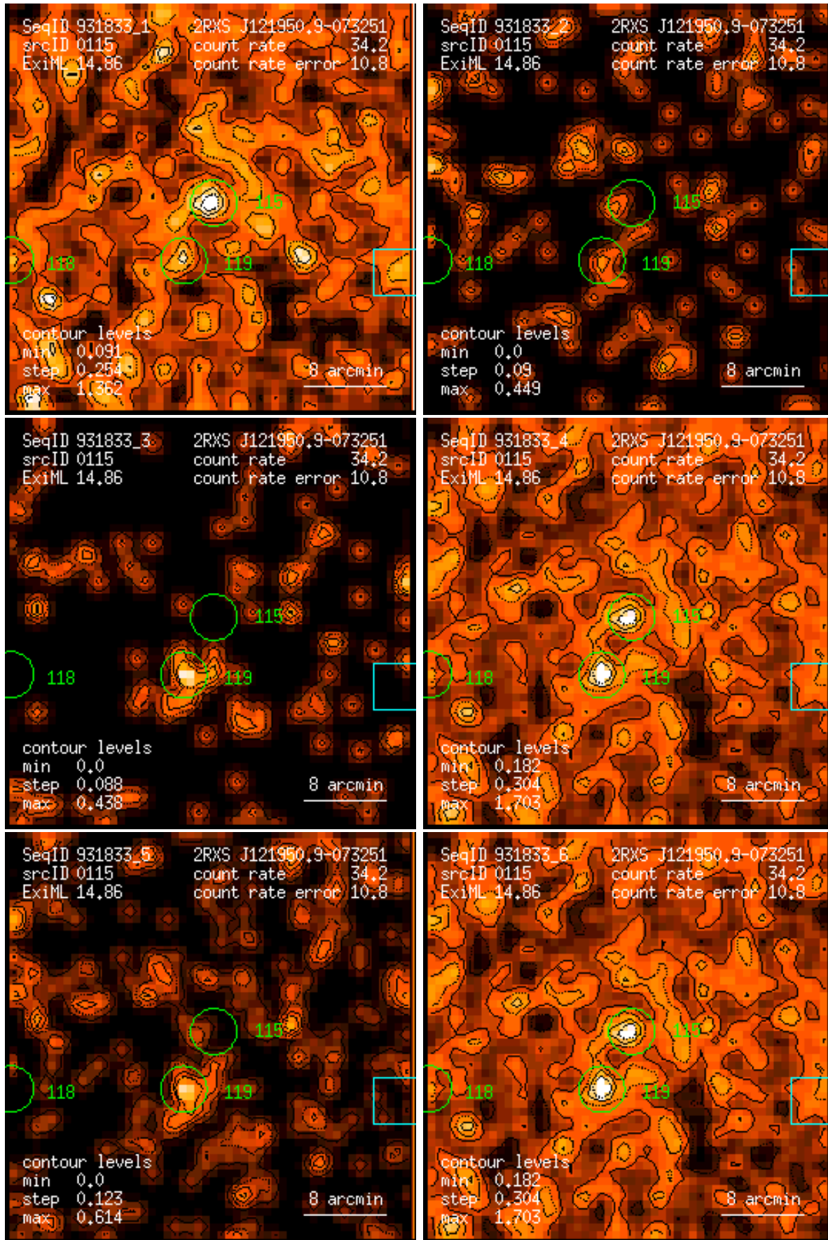
Figure 115: RASS 931833: detection 0115: band rate images, Gaussian filter: (1) PSPC channels 11 – 41, (2) 52 – 90, (3) 91 – 201, (4) 11 – 235, (5) 52 – 201, (6) 11 – 201. Broad band rates in counts/ks. Band rate contour levels in counts/ks/arcmin 2 .
