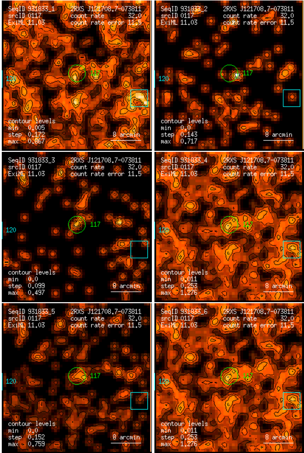
Figure 117: RASS 931833: detection 0117: band rate images, Gaussian filter: (1) PSPC channels 11 – 41, (2) 52 – 90, (3) 91 – 201, (4) 11 – 235, (5) 52 – 201, (6) 11 – 201. Broad band rates in counts/ks. Band rate contour levels in counts/ks/arcmin 2 .
