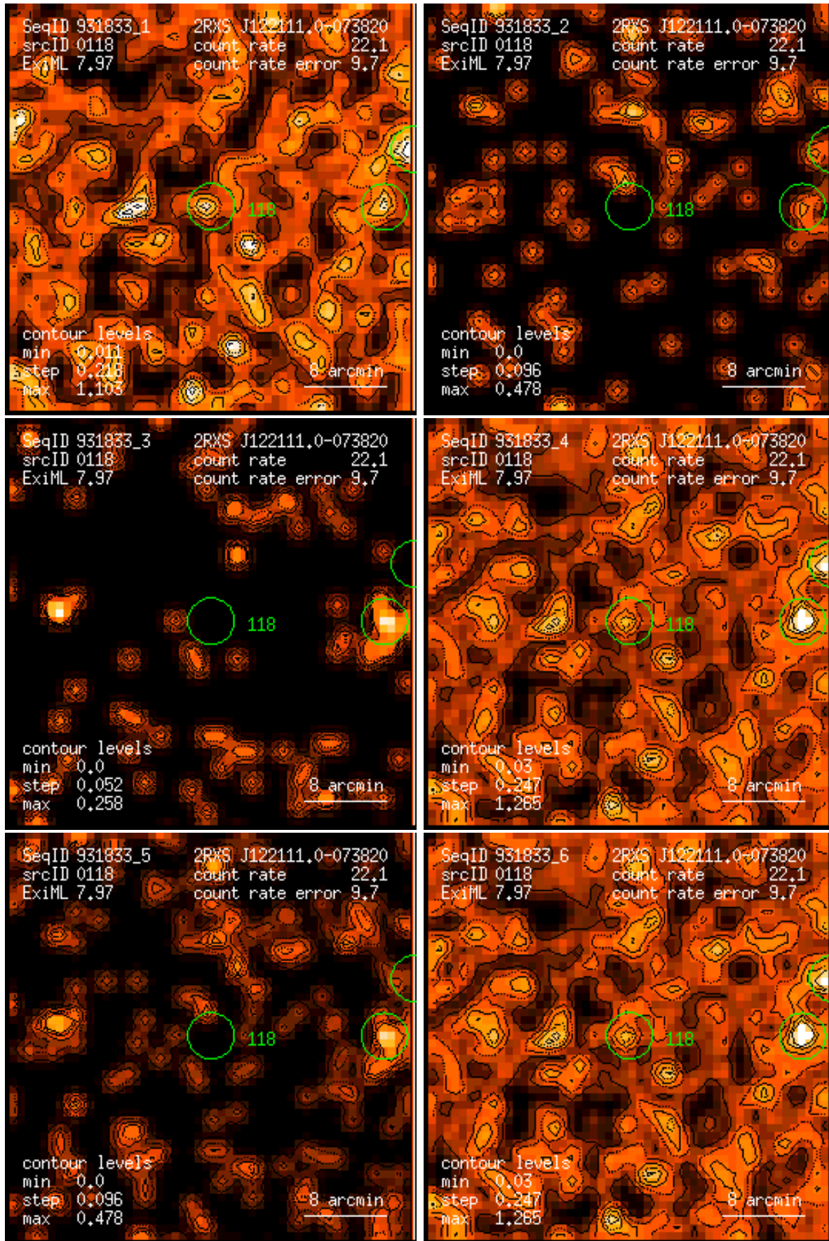
Figure 118: RASS 931833: detection 0118: band rate images, Gaussian filter: (1) PSPC channels 11 – 41, (2) 52 – 90, (3) 91 – 201, (4) 11 – 235, (5) 52 – 201, (6) 11 – 201. Broad band rates in counts/ks. Band rate contour levels in counts/ks/arcmin 2 .
