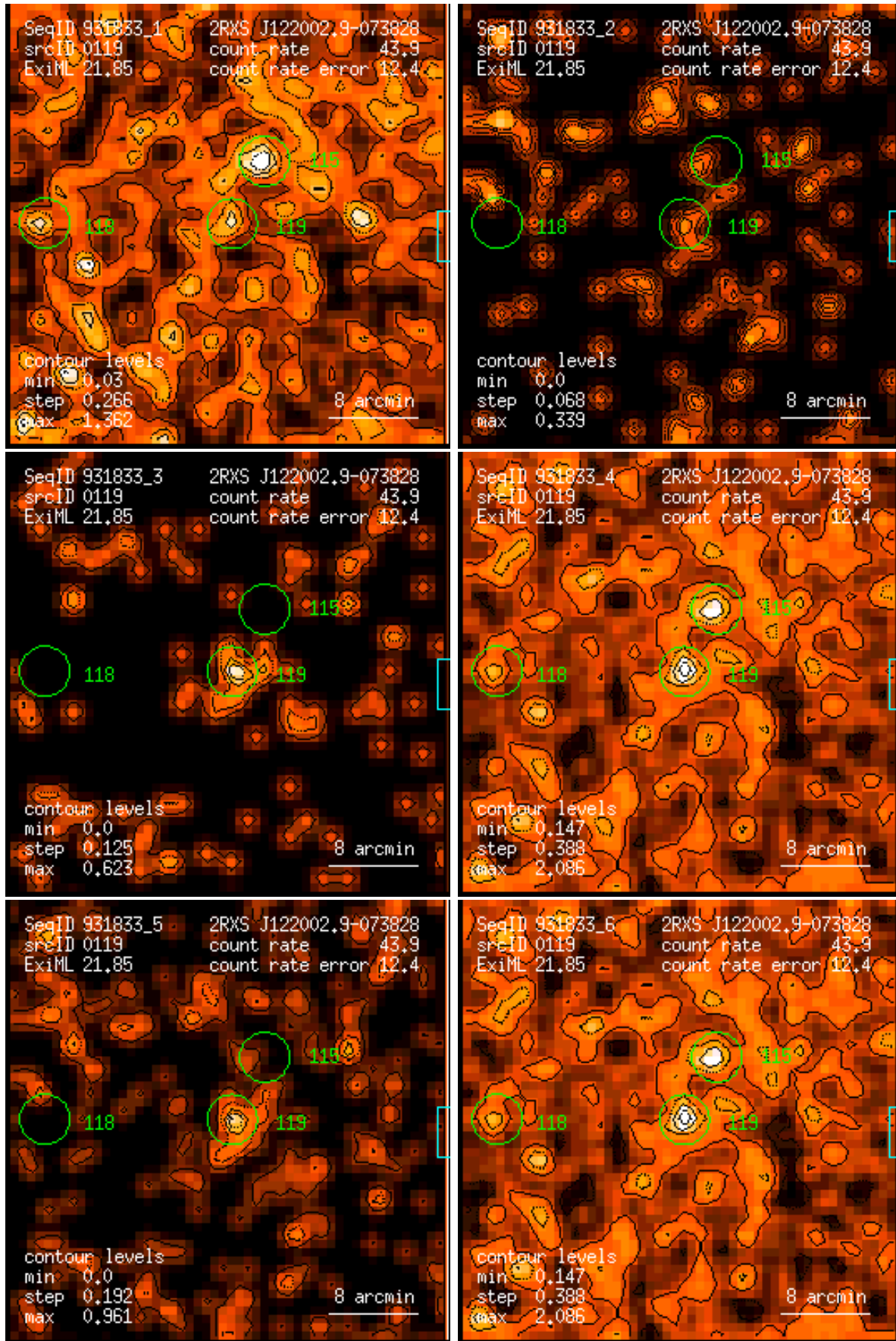
Figure 119: RASS 931833: detection 0119: band rate images, Gaussian filter: (1) PSPC channels 11 – 41, (2) 52 – 90, (3) 91 – 201, (4) 11 – 235, (5) 52 – 201, (6) 11 – 201. Broad band rates in counts/ks. Band rate contour levels in counts/ks/arcmin 2 .
