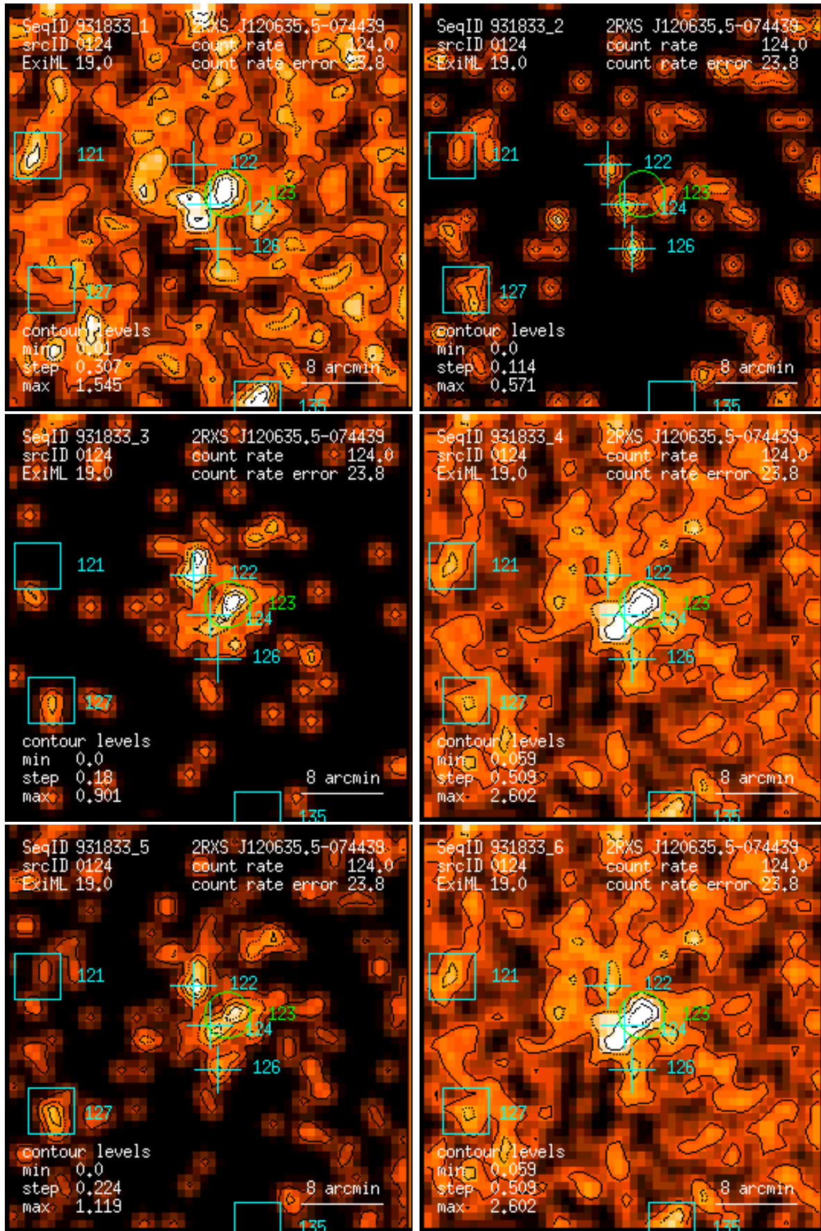
Figure 124: RASS 931833: detection 0124: band rate images, Gaussian filter: (1) PSPC channels 11 – 41, (2) 52 – 90, (3) 91 – 201, (4) 11 – 235, (5) 52 – 201, (6) 11 – 201. Broad band rates in counts/ks. Band rate contour levels in counts/ks/arcmin 2 .
