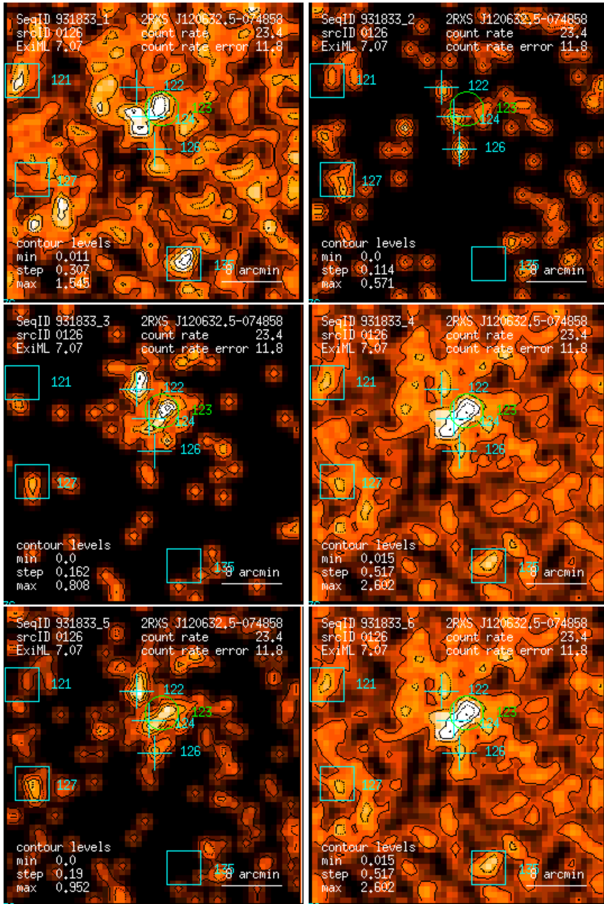
Figure 126: RASS 931833: detection 0126: band rate images, Gaussian filter: (1) PSPC channels 11 – 41, (2) 52 – 90, (3) 91 – 201, (4) 11 – 235, (5) 52 – 201, (6) 11 – 201. Broad band rates in counts/ks. Band rate contour levels in counts/ks/arcmin 2 .
