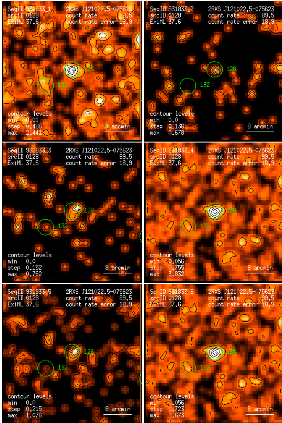
Figure 128: RASS 931833: detection 0128: band rate images, Gaussian filter: (1) PSPC channels 11 – 41, (2) 52 – 90, (3) 91 – 201, (4) 11 – 235, (5) 52 – 201, (6) 11 – 201. Broad band rates in counts/ks. Band rate contour levels in counts/ks/arcmin 2 .
