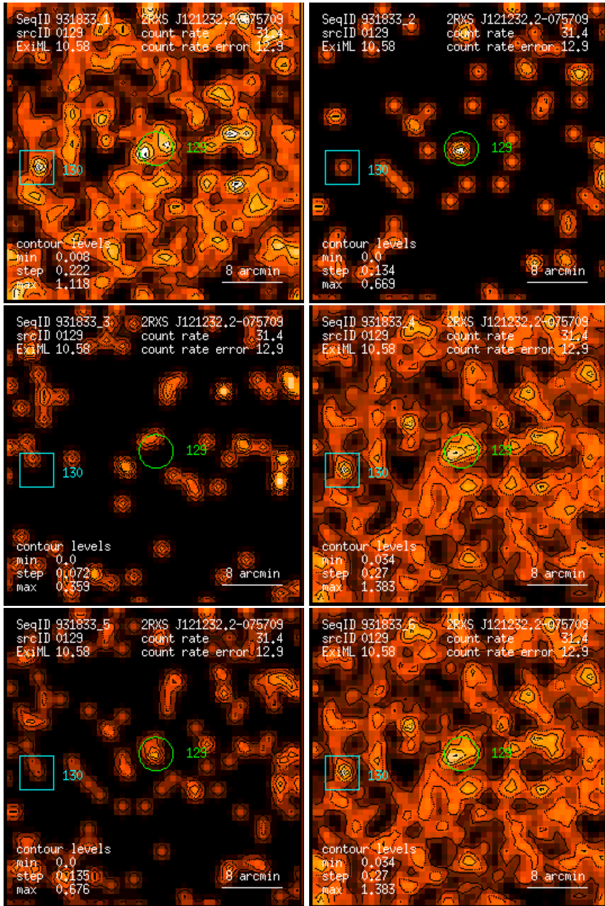
Figure 129: RASS 931833: detection 0129: band rate images, Gaussian filter: (1) PSPC channels 11 – 41, (2) 52 – 90, (3) 91 – 201, (4) 11 – 235, (5) 52 – 201, (6) 11 – 201. Broad band rates in counts/ks. Band rate contour levels in counts/ks/arcmin 2 .
