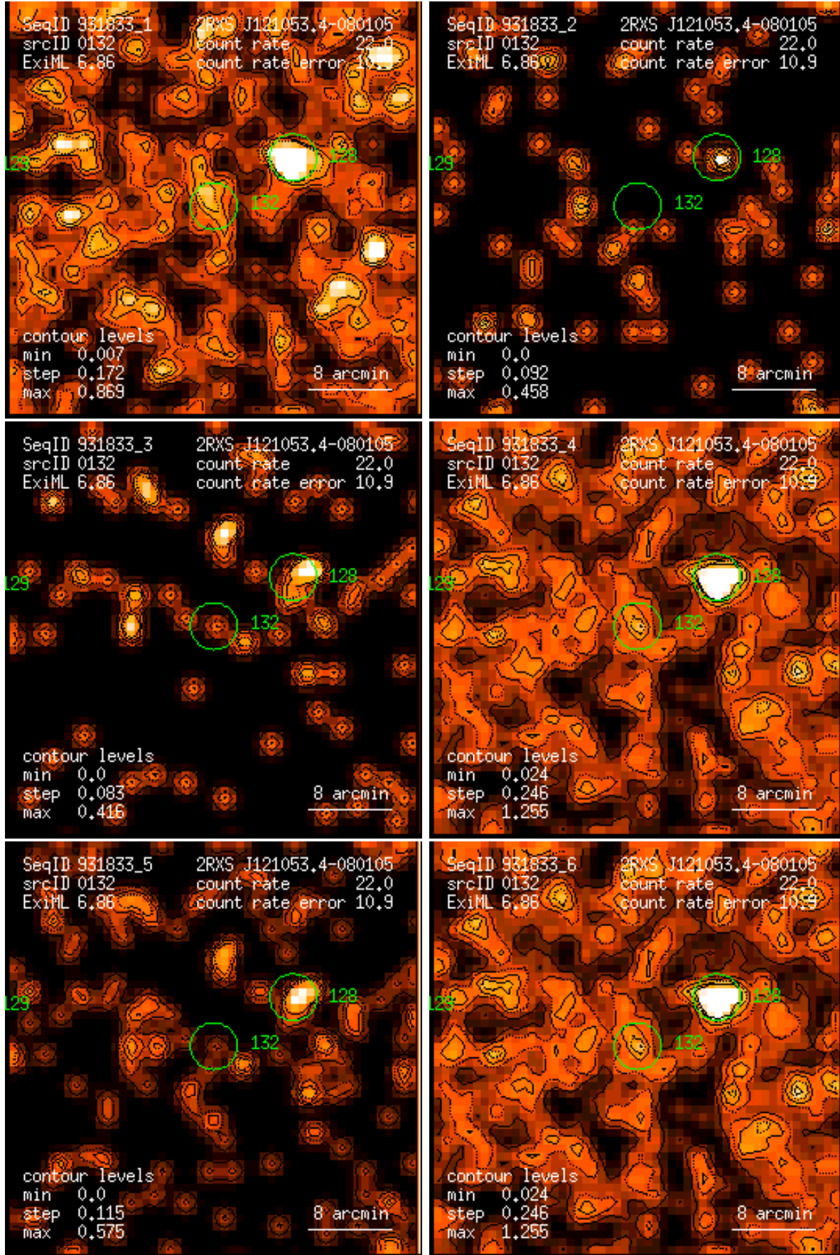
Figure 132: RASS 931833: detection 0132: band rate images, Gaussian filter: (1) PSPC channels 11 – 41, (2) 52 – 90, (3) 91 – 201, (4) 11 – 235, (5) 52 – 201, (6) 11 – 201. Broad band rates in counts/ks. Band rate contour levels in counts/ks/arcmin 2 .
