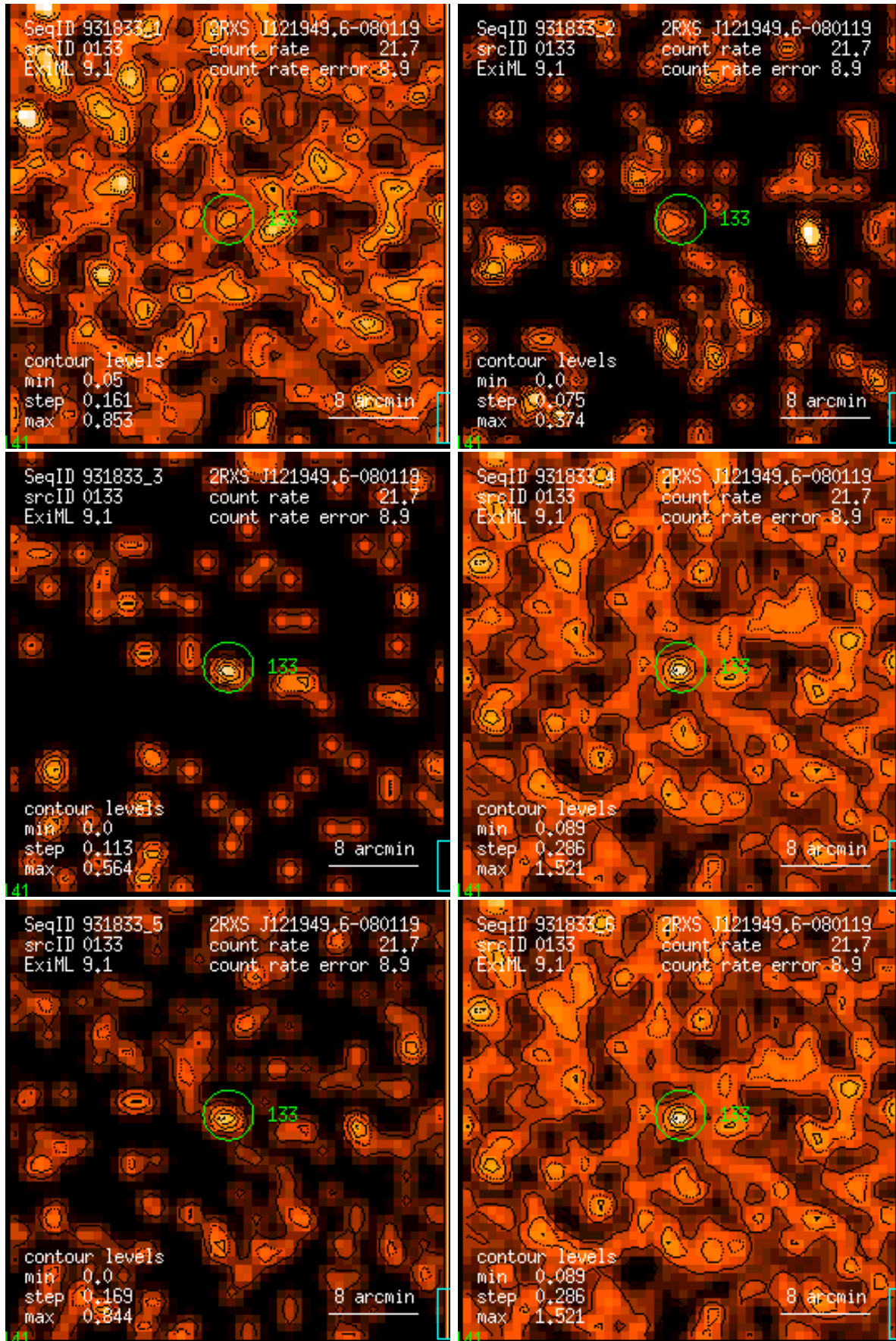
Figure 133: RASS 931833: detection 0133: band rate images, Gaussian filter: (1) PSPC channels 11 – 41, (2) 52 – 90, (3) 91 – 201, (4) 11 – 235, (5) 52 – 201, (6) 11 – 201. Broad band rates in counts/ks. Band rate contour levels in counts/ks/arcmin 2 .
