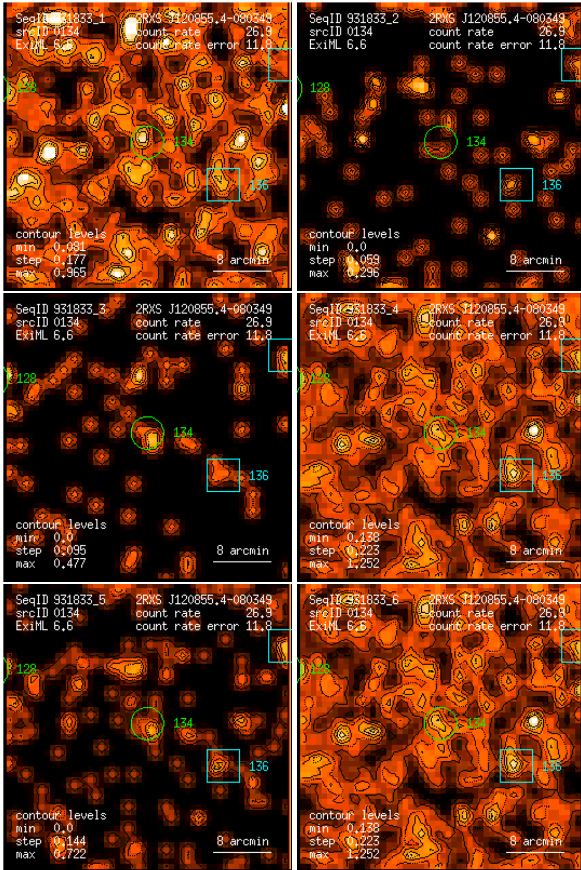
Figure 134: RASS 931833: detection 0134: band rate images, Gaussian filter: (1) PSPC channels 11 – 41, (2) 52 – 90, (3) 91 – 201, (4) 11 – 235, (5) 52 – 201, (6) 11 – 201. Broad band rates in counts/ks. Band rate contour levels in counts/ks/arcmin 2 .
