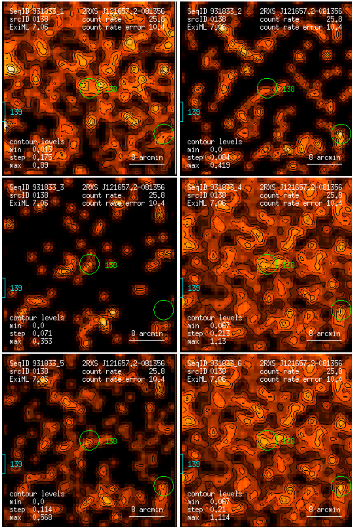
Figure 138: RASS 931833: detection 0138: band rate images, Gaussian filter: (1) PSPC channels 11 – 41, (2) 52 – 90, (3) 91 – 201, (4) 11 – 235, (5) 52 – 201, (6) 11 – 201. Broad band rates in counts/ks. Band rate contour levels in counts/ks/arcmin 2 .
