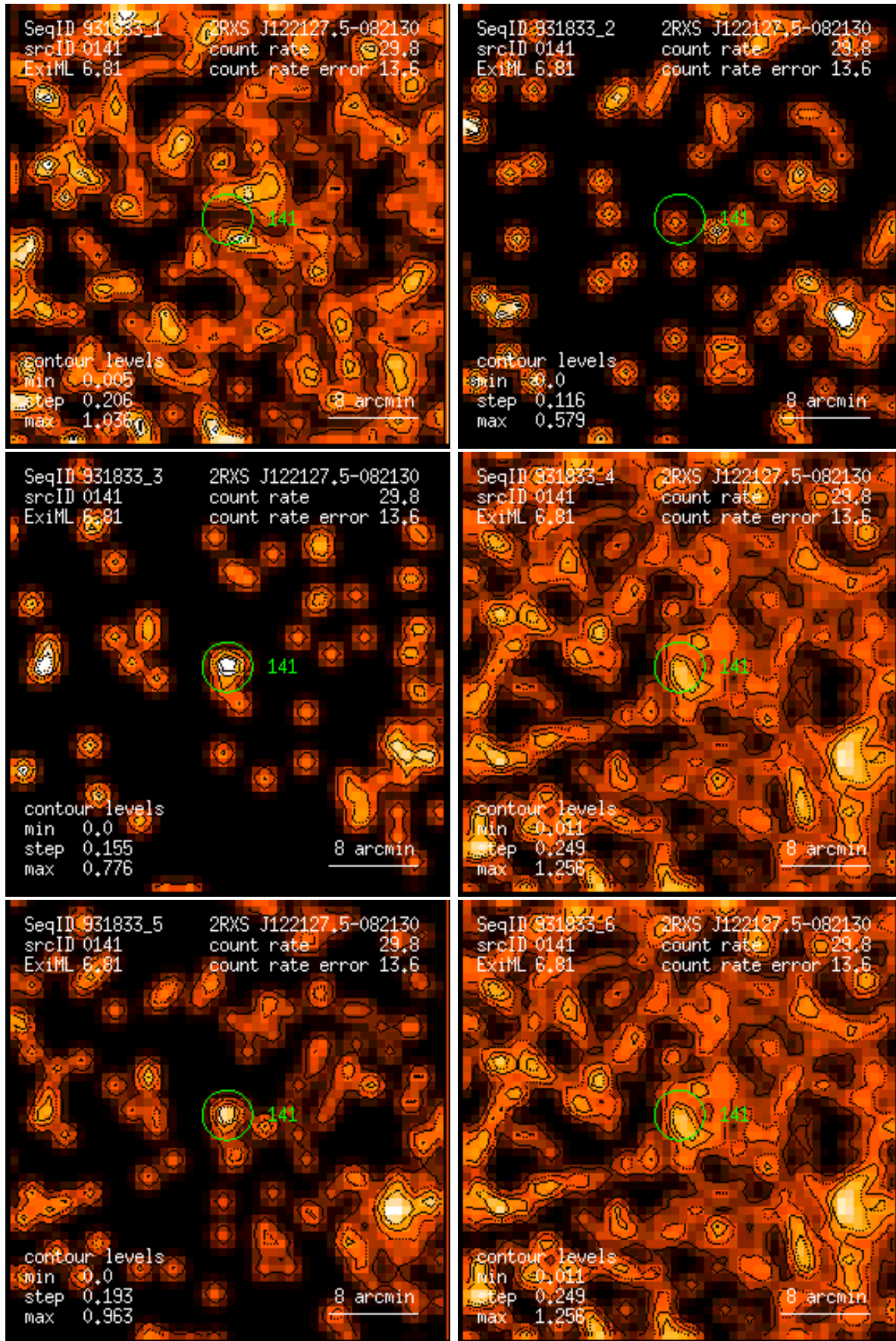
Figure 141: RASS 931833: detection 0141: band rate images, Gaussian filter: (1) PSPC channels 11 – 41, (2) 52 – 90, (3) 91 – 201, (4) 11 – 235, (5) 52 – 201, (6) 11 – 201. Broad band rates in counts/ks. Band rate contour levels in counts/ks/arcmin 2 .
