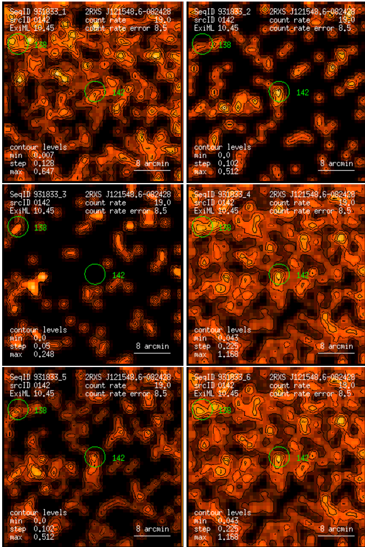
Figure 142: RASS 931833: detection 0142: band rate images, Gaussian filter: (1) PSPC channels 11 – 41, (2) 52 – 90, (3) 91 – 201, (4) 11 – 235, (5) 52 – 201, (6) 11 – 201. Broad band rates in counts/ks. Band rate contour levels in counts/ks/arcmin 2 .
