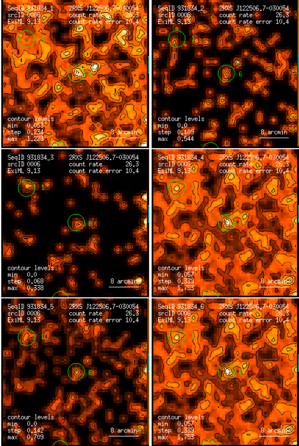
Figure 6: RASS 931834: detection 0006: band rate images, Gaussian filter: (1) PSPC channels 11 – 41, (2) 52 – 90, (3) 91 – 201, (4) 11 – 235, (5) 52 – 201, (6) 11 – 201. Broad band rates in counts/ks. Band rate contour levels in counts/ks/arcmin 2 .
