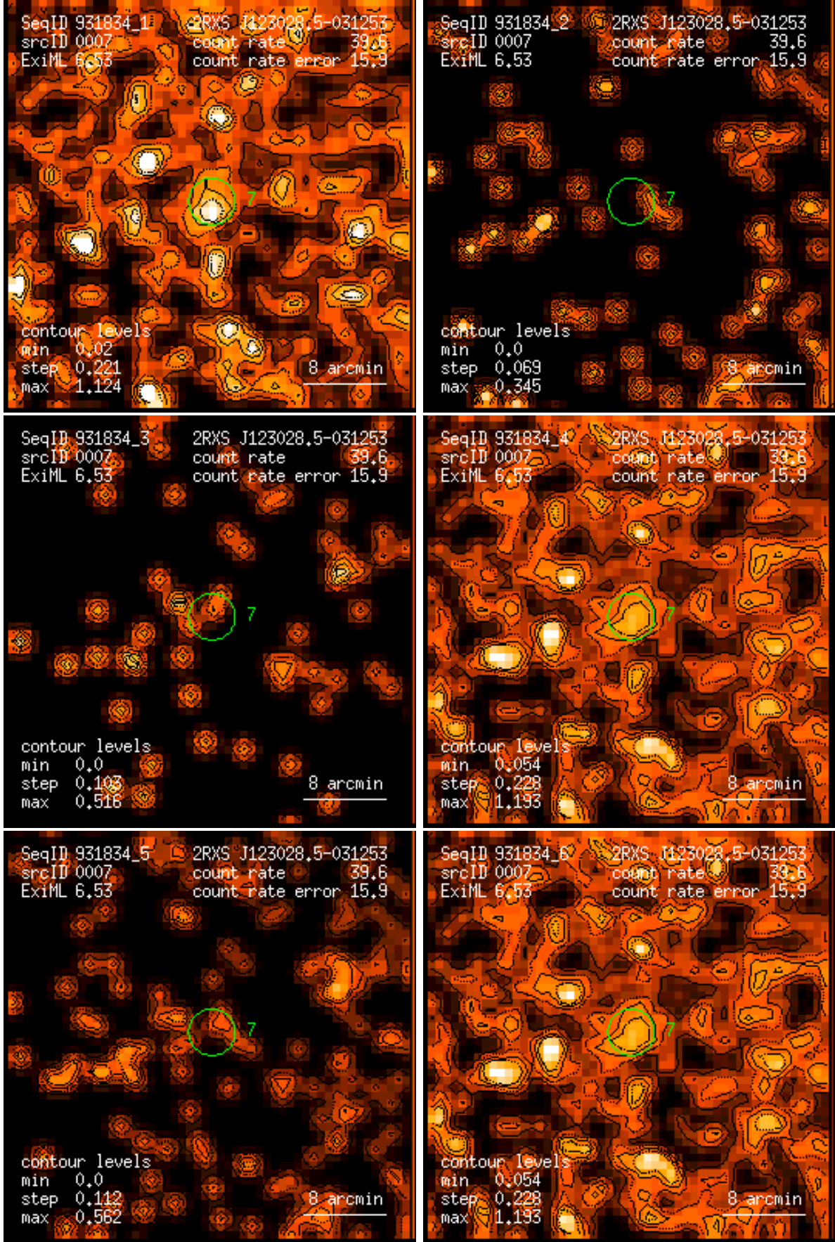
Figure 7: RASS 931834: detection 0007: band rate images, Gaussian filter: (1) PSPC channels 11 – 41, (2) 52 – 90, (3) 91 – 201, (4) 11 – 235, (5) 52 – 201, (6) 11 – 201. Broad band rates in counts/ks. Band rate contour levels in counts/ks/arcmin 2 .
