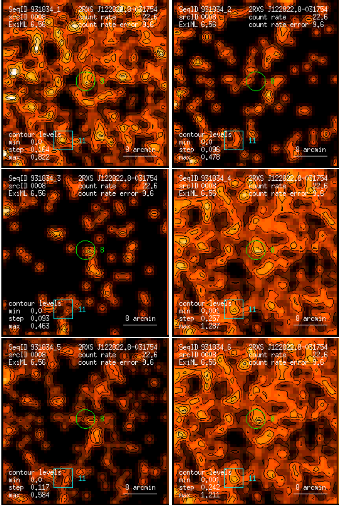
Figure 8: RASS 931834: detection 0008: band rate images, Gaussian filter: (1) PSPC channels 11 – 41, (2) 52 – 90, (3) 91 – 201, (4) 11 – 235, (5) 52 – 201, (6) 11 – 201. Broad band rates in counts/ks. Band rate contour levels in counts/ks/arcmin 2 .
