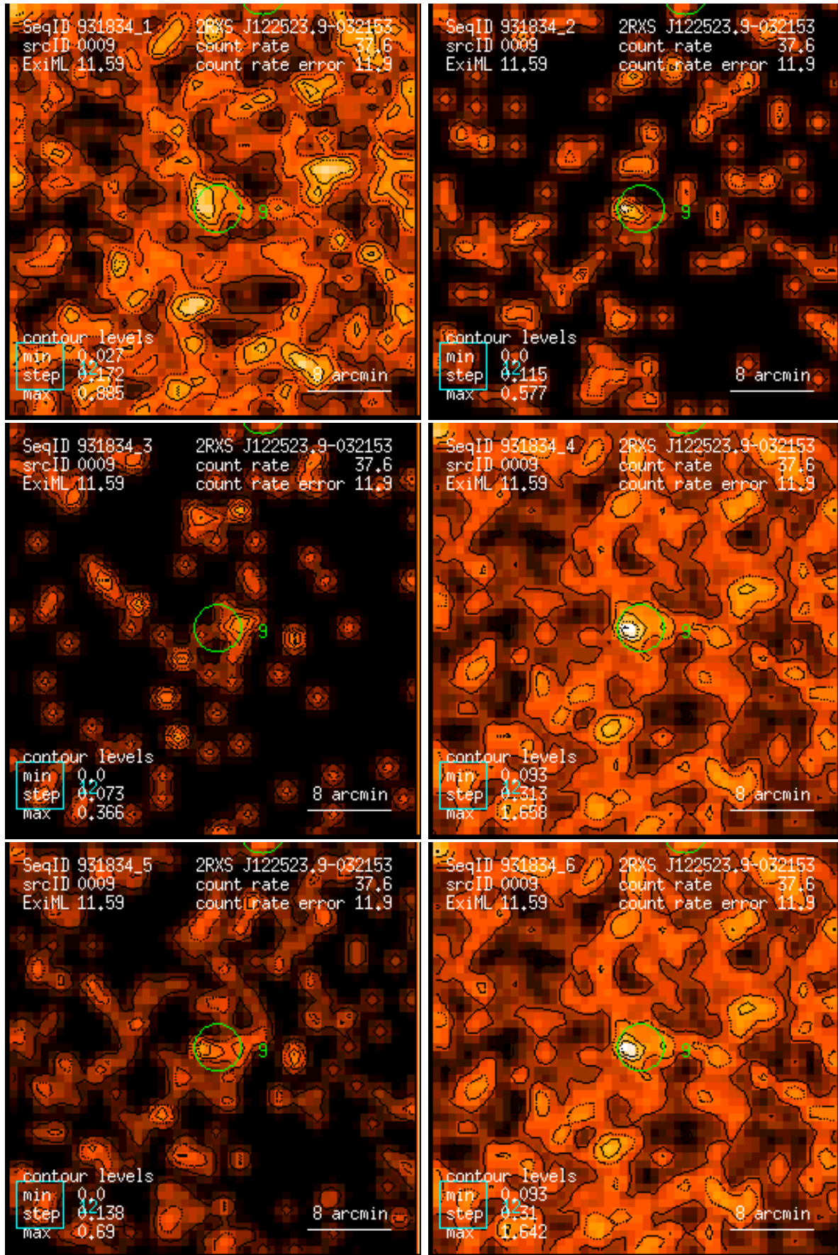
Figure 9: RASS 931834: detection 0009: band rate images, Gaussian filter: (1) PSPC channels 11 – 41, (2) 52 – 90, (3) 91 – 201, (4) 11 – 235, (5) 52 – 201, (6) 11 – 201. Broad band rates in counts/ks. Band rate contour levels in counts/ks/arcmin 2 .
