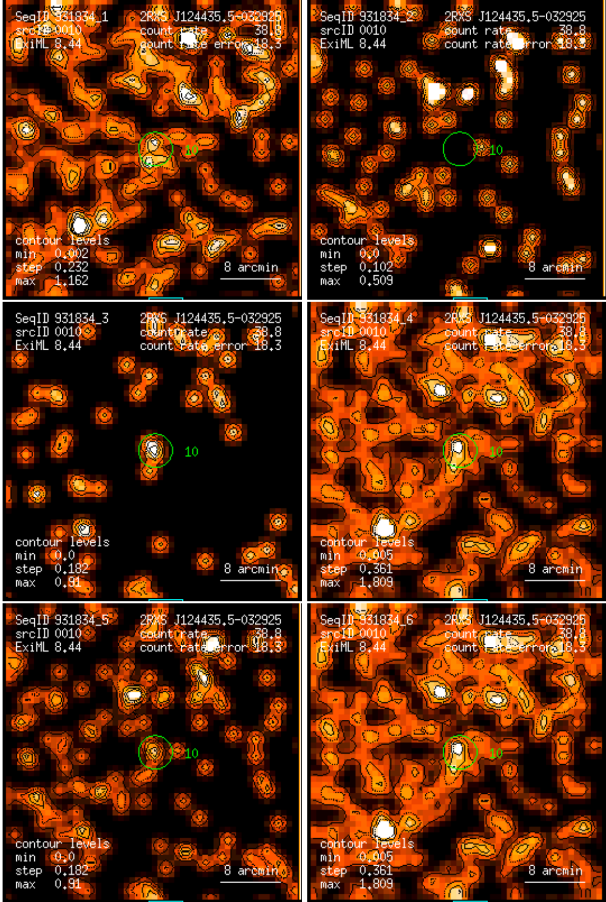
Figure 10: RASS 931834: detection 0010: band rate images, Gaussian filter: (1) PSPC channels 11 – 41, (2) 52 – 90, (3) 91 – 201, (4) 11 – 235, (5) 52 – 201, (6) 11 – 201. Broad band rates in counts/ks. Band rate contour levels in counts/ks/arcmin 2 .
