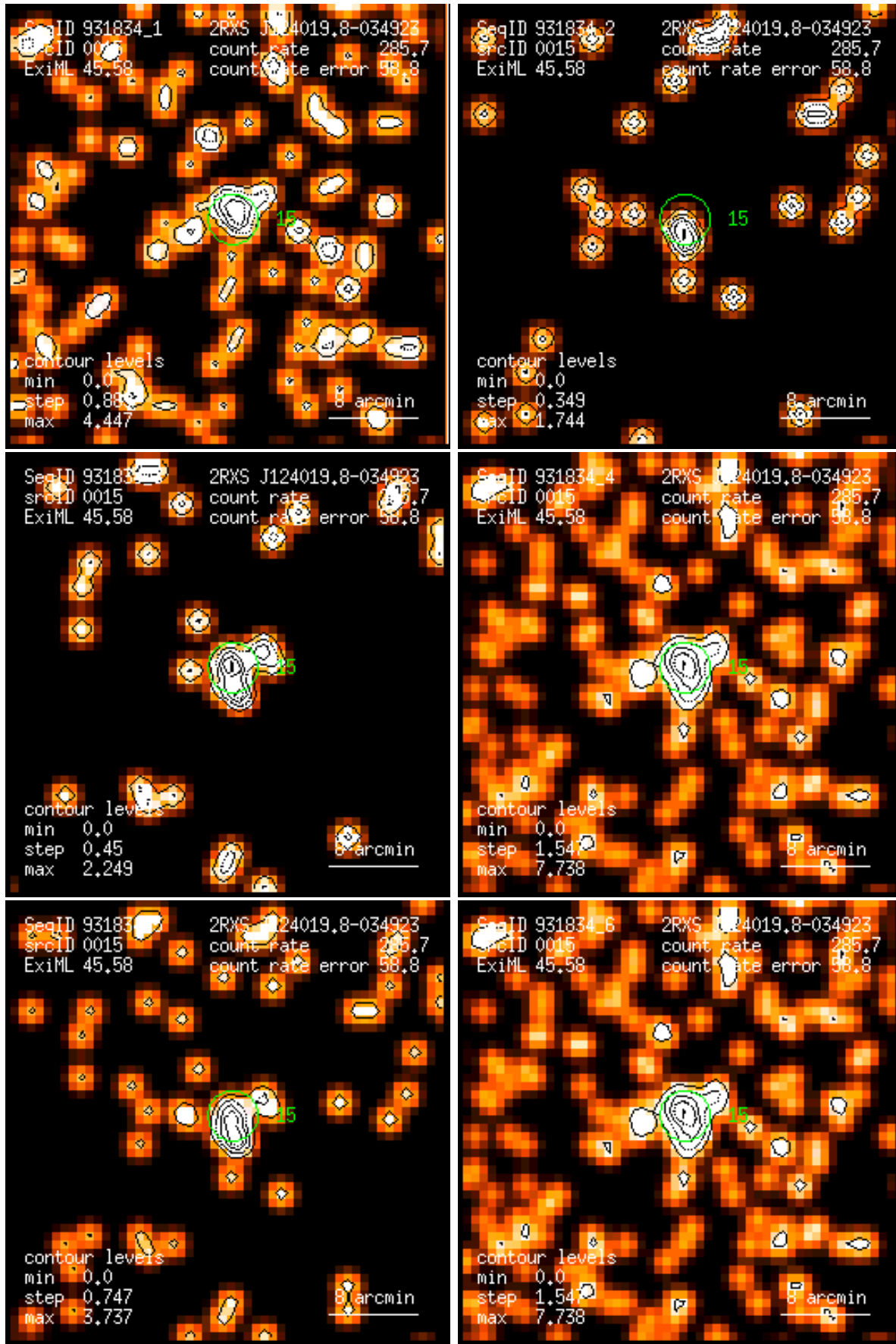
Figure 15: RASS 931834: detection 0015: band rate images, Gaussian filter: (1) PSPC channels 11 – 41, (2) 52 – 90, (3) 91 – 201, (4) 11 – 235, (5) 52 – 201, (6) 11 – 201. Broad band rates in counts/ks. Band rate contour levels in counts/ks/arcmin 2 .
