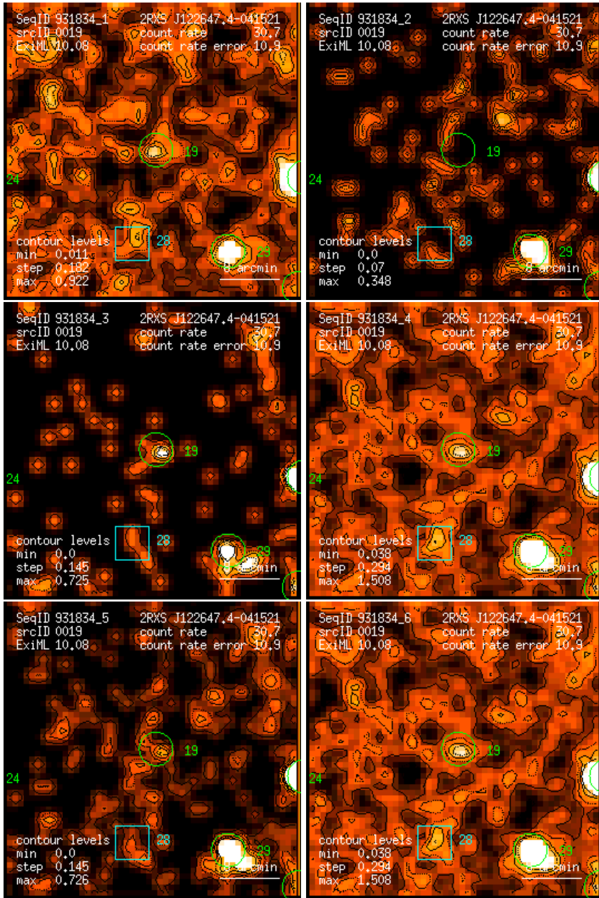
Figure 19: RASS 931834: detection 0019: band rate images, Gaussian filter: (1) PSPC channels 11 – 41, (2) 52 – 90, (3) 91 – 201, (4) 11 – 235, (5) 52 – 201, (6) 11 – 201. Broad band rates in counts/ks. Band rate contour levels in counts/ks/arcmin 2 .
