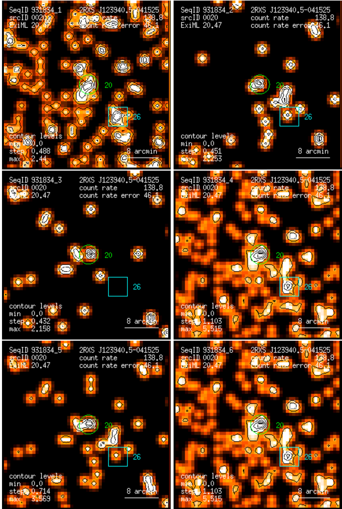
Figure 20: RASS 931834: detection 0020: band rate images, Gaussian filter: (1) PSPC channels 11 – 41, (2) 52 – 90, (3) 91 – 201, (4) 11 – 235, (5) 52 – 201, (6) 11 – 201. Broad band rates in counts/ks. Band rate contour levels in counts/ks/arcmin 2 .
