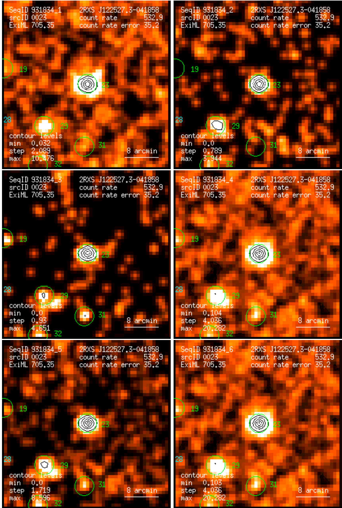
Figure 23: RASS 931834: detection 0023: band rate images, Gaussian filter: (1) PSPC channels 11 – 41, (2) 52 – 90, (3) 91 – 201, (4) 11 – 235, (5) 52 – 201, (6) 11 – 201. Broad band rates in counts/ks. Band rate contour levels in counts/ks/arcmin 2 .
