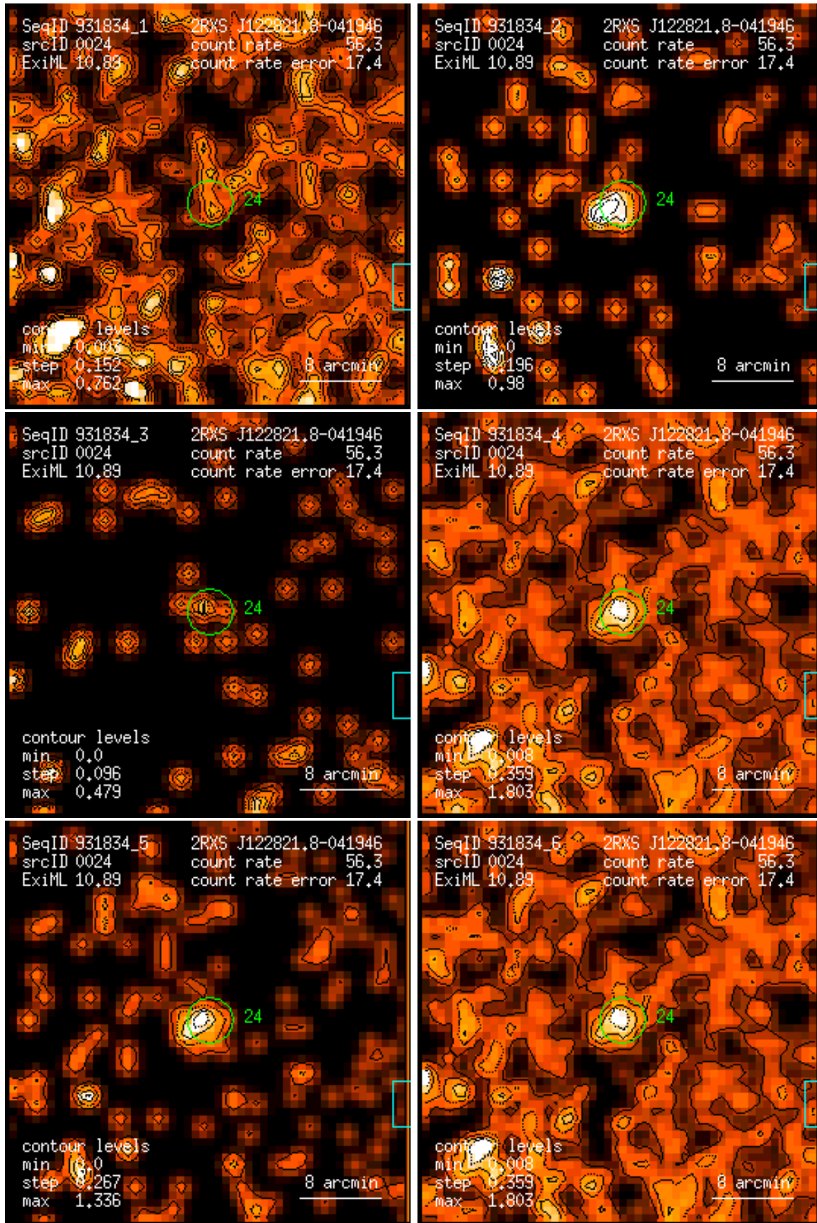
Figure 24: RASS 931834: detection 0024: band rate images, Gaussian filter: (1) PSPC channels 11 – 41, (2) 52 – 90, (3) 91 – 201, (4) 11 – 235, (5) 52 – 201, (6) 11 – 201. Broad band rates in counts/ks. Band rate contour levels in counts/ks/arcmin 2 .
