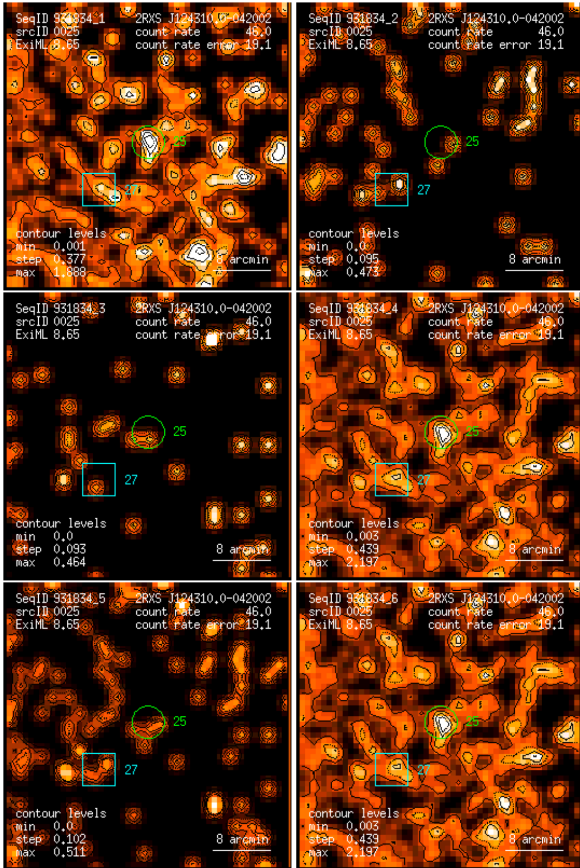
Figure 25: RASS 931834: detection 0025: band rate images, Gaussian filter: (1) PSPC channels 11 – 41, (2) 52 – 90, (3) 91 – 201, (4) 11 – 235, (5) 52 – 201, (6) 11 – 201. Broad band rates in counts/ks. Band rate contour levels in counts/ks/arcmin 2 .
