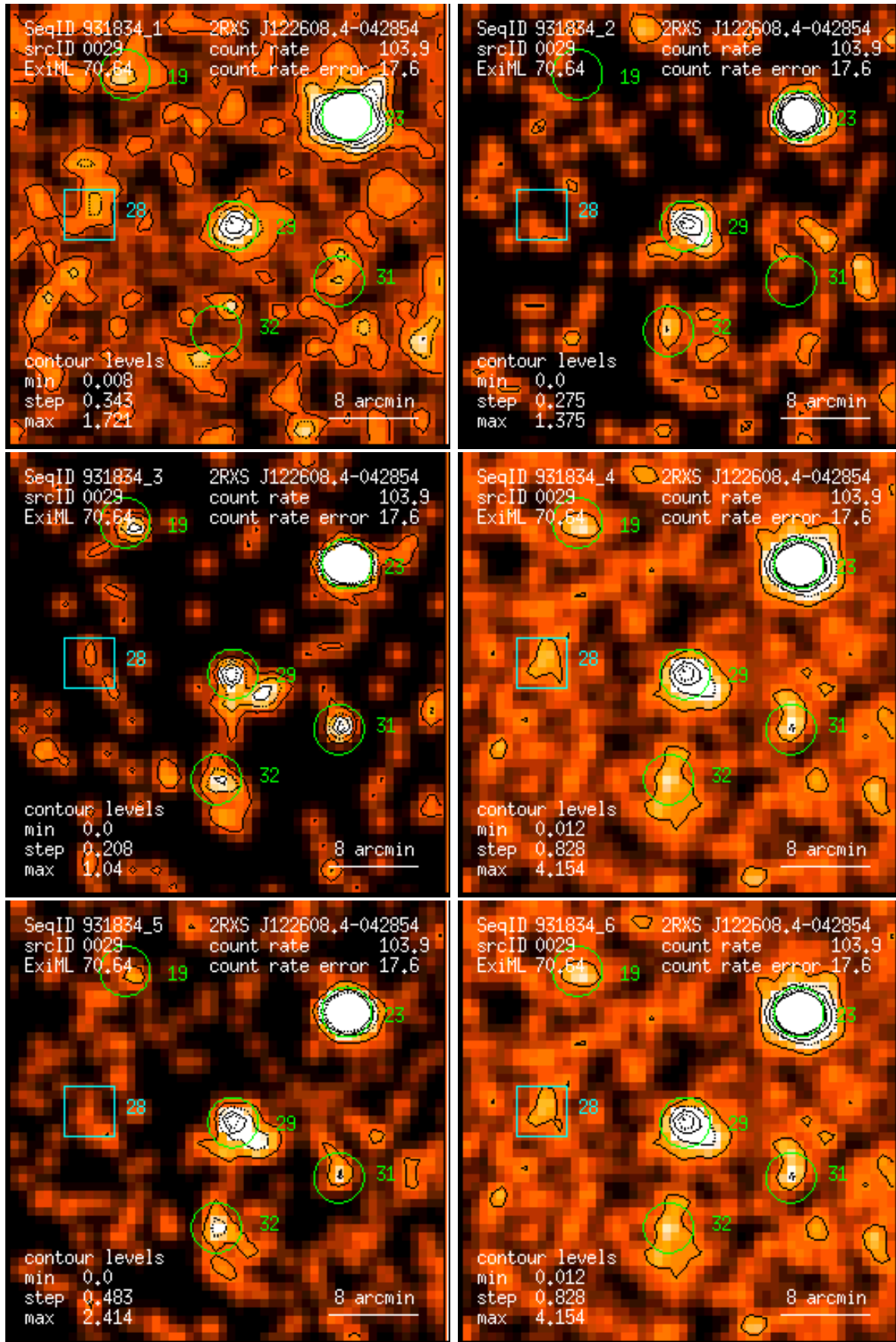
Figure 29: RASS 931834: detection 0029: band rate images, Gaussian filter: (1) PSPC channels 11 – 41, (2) 52 – 90, (3) 91 – 201, (4) 11 – 235, (5) 52 – 201, (6) 11 – 201. Broad band rates in counts/ks. Band rate contour levels in counts/ks/arcmin 2 .
