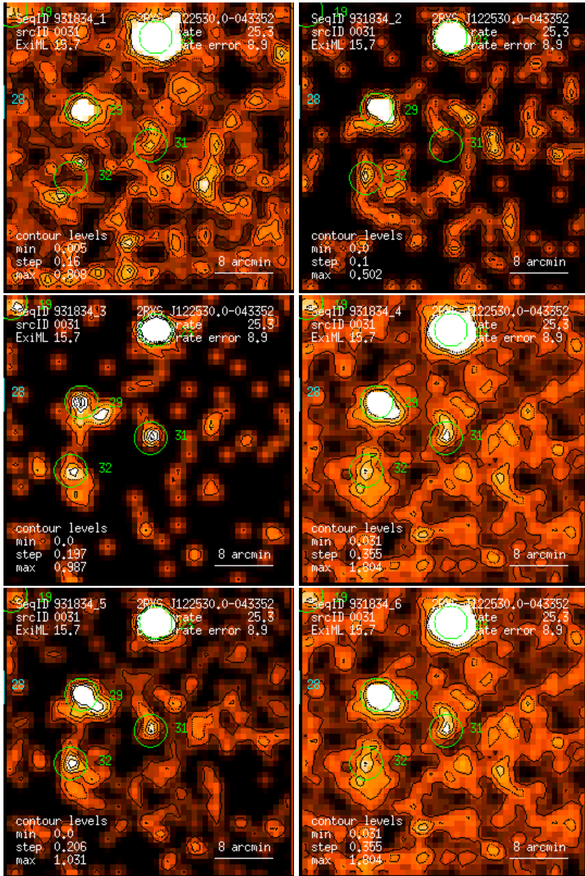
Figure 31: RASS 931834: detection 0031: band rate images, Gaussian filter: (1) PSPC channels 11 – 41, (2) 52 – 90, (3) 91 – 201, (4) 11 – 235, (5) 52 – 201, (6) 11 – 201. Broad band rates in counts/ks. Band rate contour levels in counts/ks/arcmin 2 .
