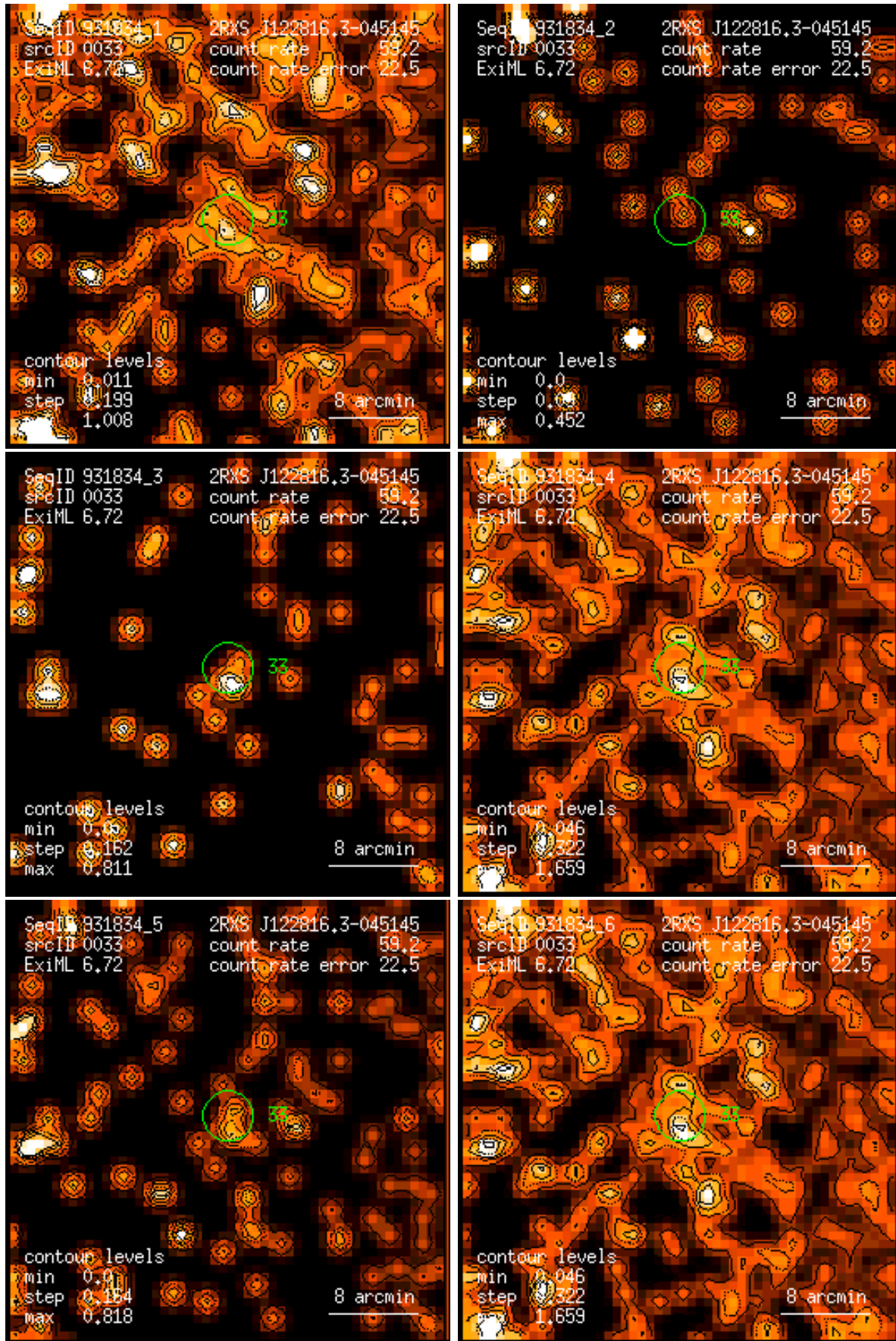
Figure 33: RASS 931834: detection 0033: band rate images, Gaussian filter: (1) PSPC channels 11 – 41, (2) 52 – 90, (3) 91 – 201, (4) 11 – 235, (5) 52 – 201, (6) 11 – 201. Broad band rates in counts/ks. Band rate contour levels in counts/ks/arcmin 2 .
