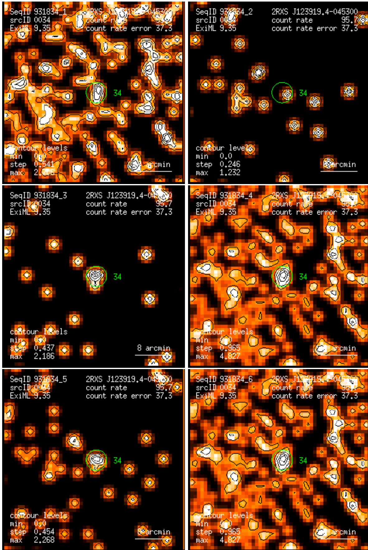
Figure 34: RASS 931834: detection 0034: band rate images, Gaussian filter: (1) PSPC channels 11 – 41, (2) 52 – 90, (3) 91 – 201, (4) 11 – 235, (5) 52 – 201, (6) 11 – 201. Broad band rates in counts/ks. Band rate contour levels in counts/ks/arcmin 2 .
