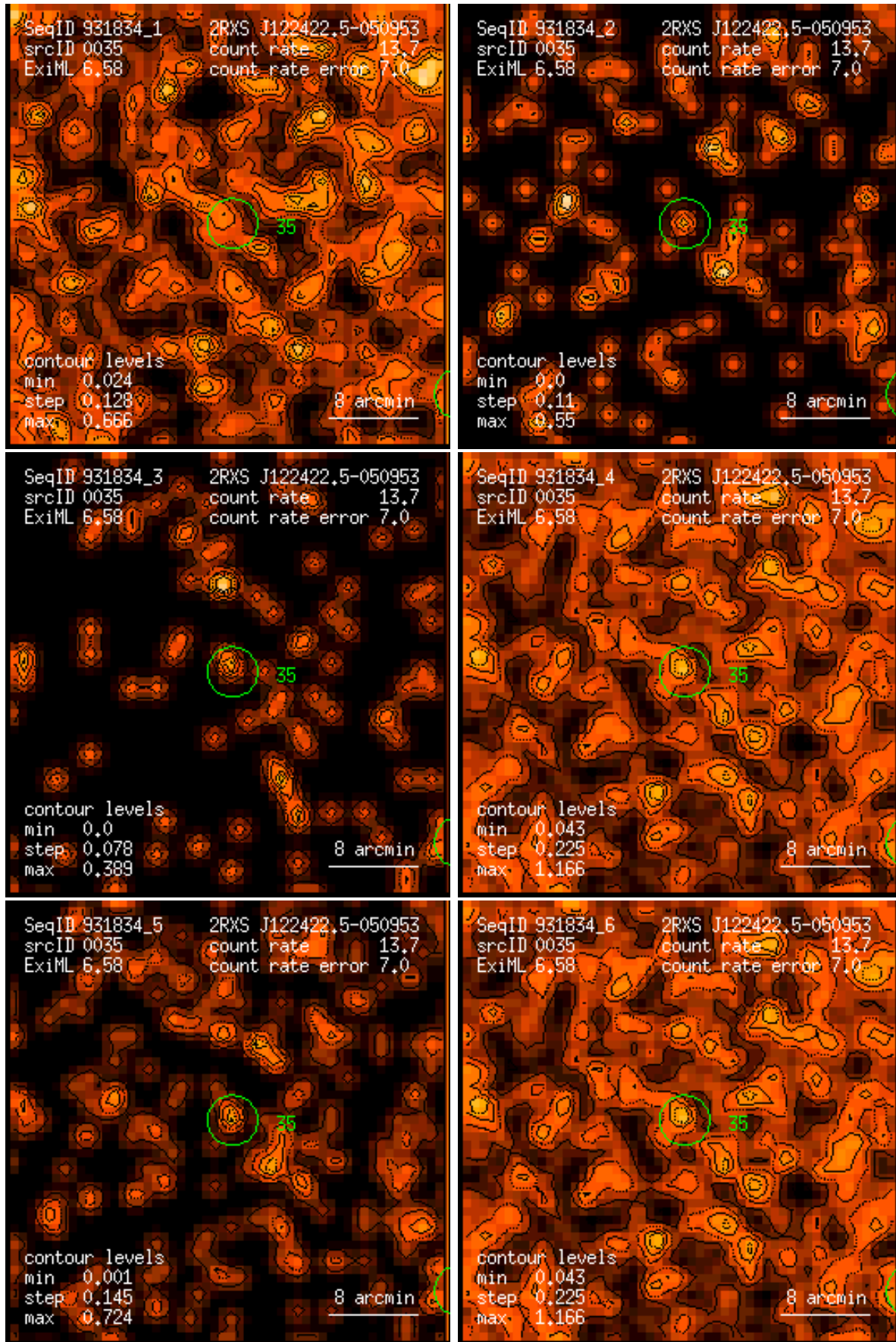
Figure 35: RASS 931834: detection 0035: band rate images, Gaussian filter: (1) PSPC channels 11 – 41, (2) 52 – 90, (3) 91 – 201, (4) 11 – 235, (5) 52 – 201, (6) 11 – 201. Broad band rates in counts/ks. Band rate contour levels in counts/ks/arcmin 2 .
