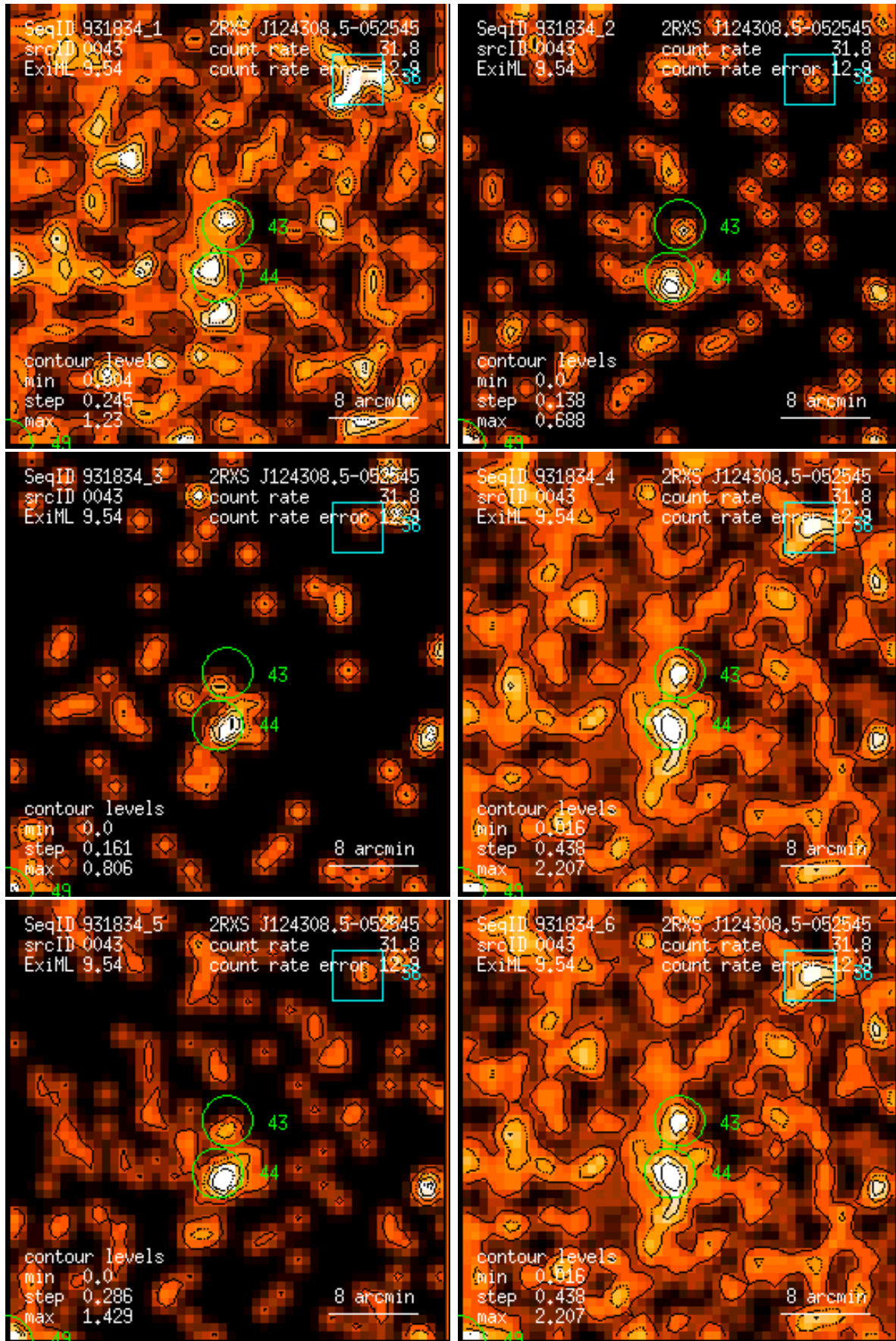
Figure 43: RASS 931834: detection 0043: band rate images, Gaussian filter: (1) PSPC channels 11 – 41, (2) 52 – 90, (3) 91 – 201, (4) 11 – 235, (5) 52 – 201, (6) 11 – 201. Broad band rates in counts/ks. Band rate contour levels in counts/ks/arcmin 2 .
